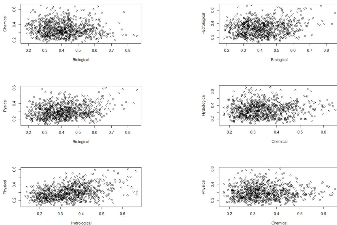
Figure. 10: Scatter graphs showing the dissimilarity between different river pairs in different clustering categories. All dissimilarity measurers were created using the Gower dissimilarity matrix with the Vegan package on R. full statistical results are shown in table. 16. However, BP, HP and BH are all statistically significantly correlated with an alpha value of below 0.05.
