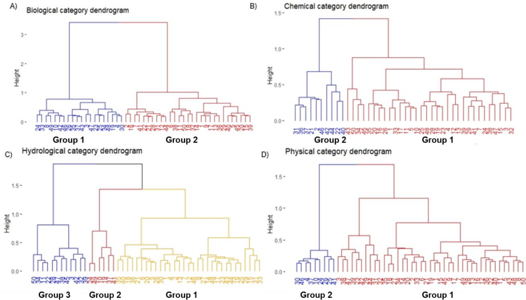
Figure. 4: Dendrogram clusters made up with the different categorical variables. The decision on where to cut the trees for groups was based on average silhouette width with the point of most explanation being chosen as the most descriptive grouping system. The case numbers refer to the same rivers in each example.
