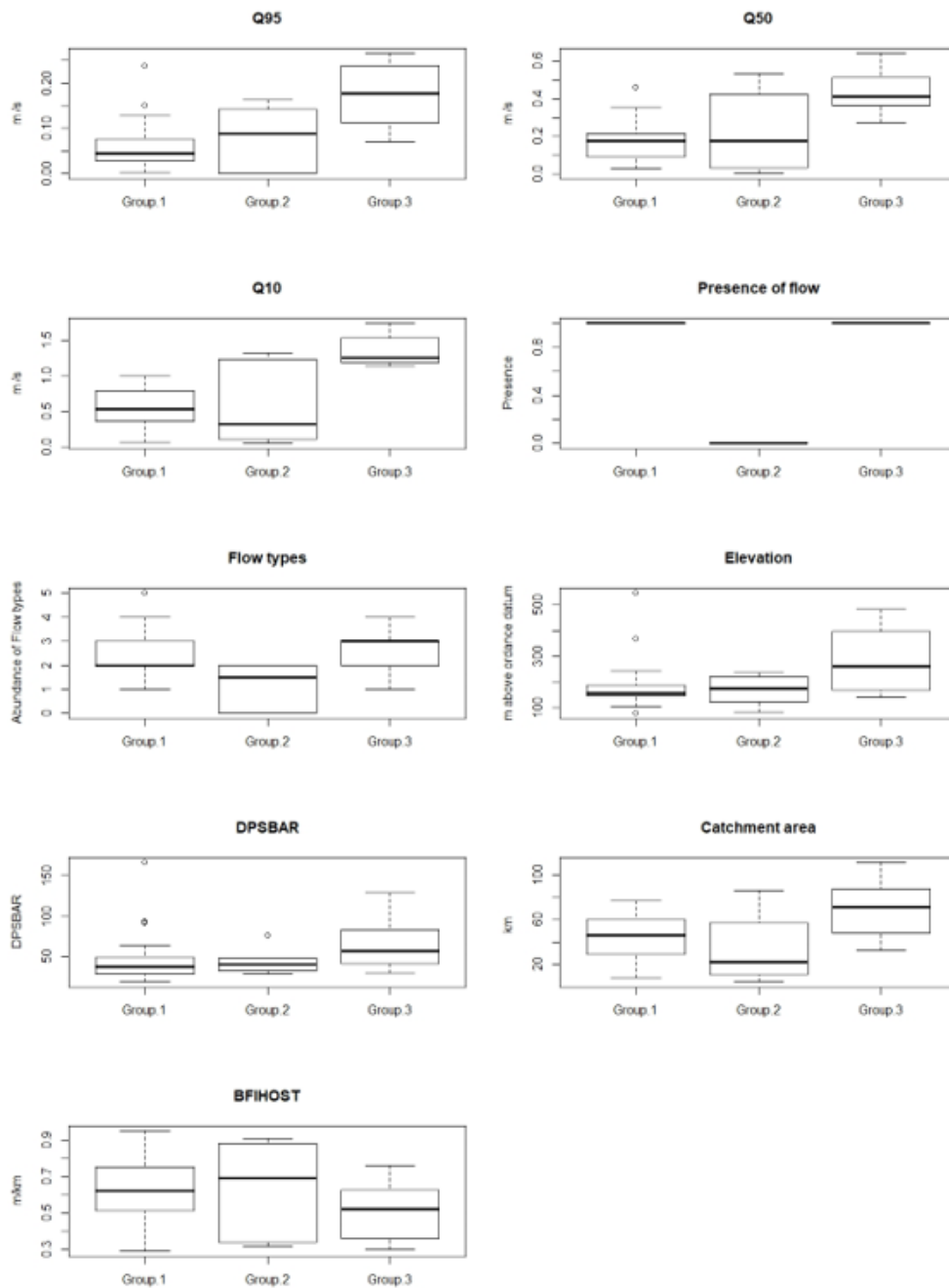
Figure. 7: Box plots showing the difference in hydrological cluster groups. Group 1 appears to be the hydrologically average river group, group 2 has all the low flow events and smaller catchment areas and group 3 has the higher catchment areas and higher flows. Data collected in the field and from the NRFA gauging system. Group 1 N=31, Group 2 N=6 and Group 3 N=12.
