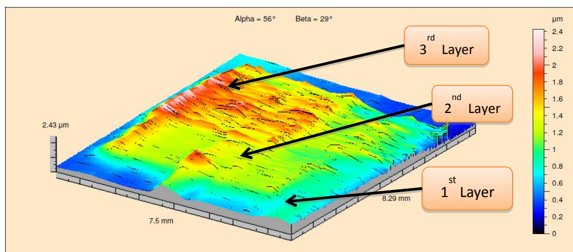
Figure 4.16: Surface profile of a PCL square sample printed at 30°C substrate with 40 \mu\text{m} droplet spacing.
