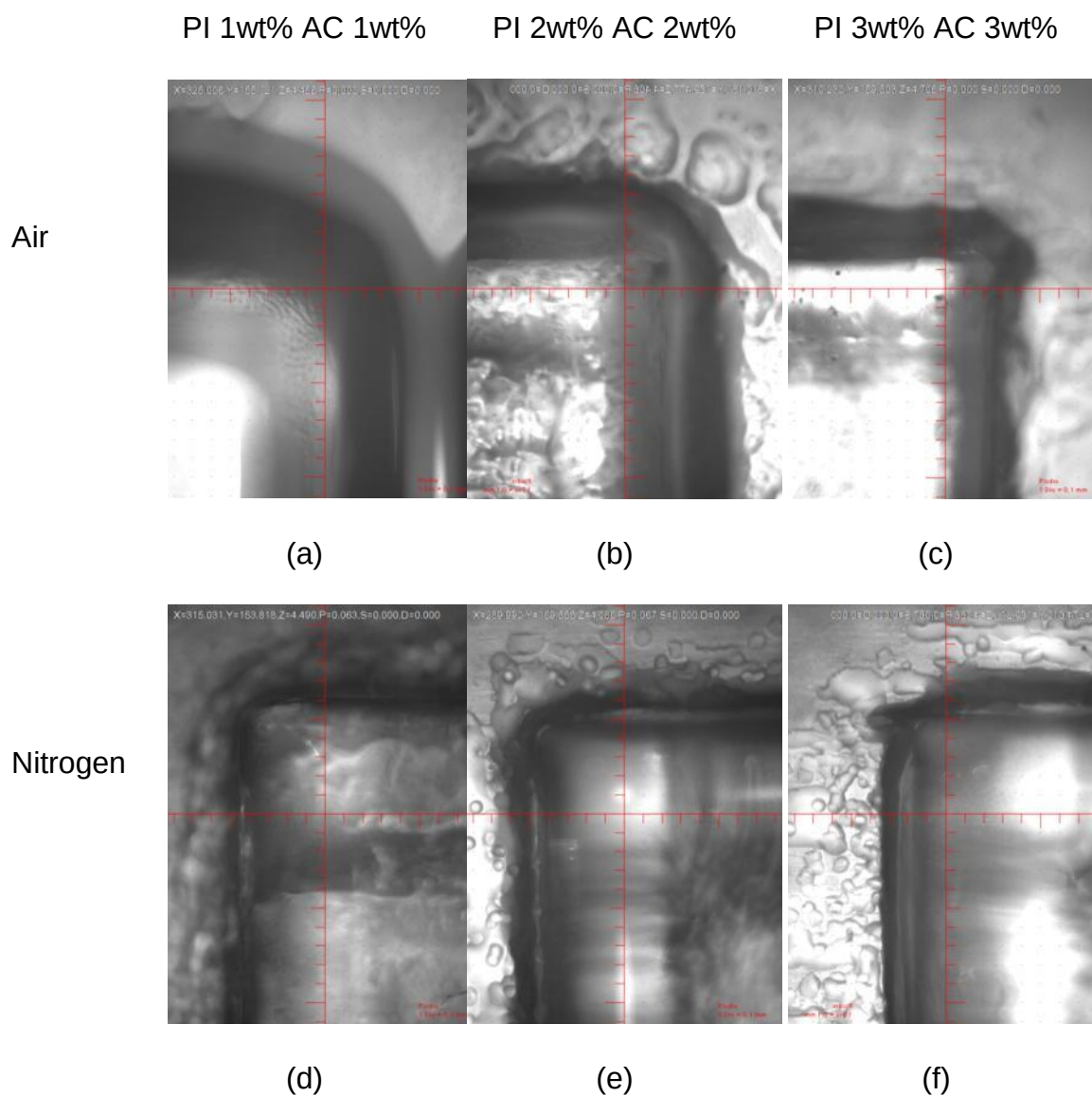
Figure 5.28: Optical microscope pictures of square samples printed with inks with different concentration of photoinitiators (PI) and accelerators (AC) in both air and nitrogen environments.(1 division=100 \mu m)
