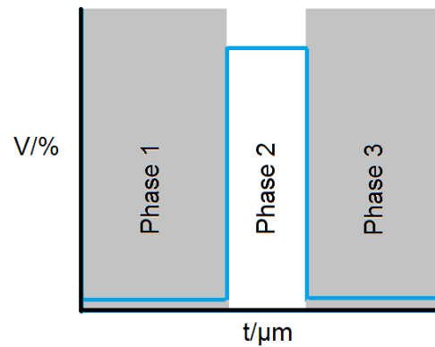
Figure 3.14: An example of a basic waveform used for a piezo actuator based DoD printhead
