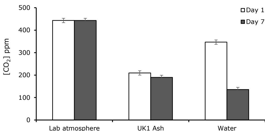
Figure 4-3: CO 2 evolution from UK1 fly ash sample on day 1 and after 7 days of fly ash incubation in comparison to the CO 2 concentration in the laboratory atmosphere and in the headspace above water. Ash and water samples were maintained in closed airtight serum bottles. Individual error bars are based on the pooled variance estimate from the ANOVA with 12 degrees of freedom. LSD = 29.84.
