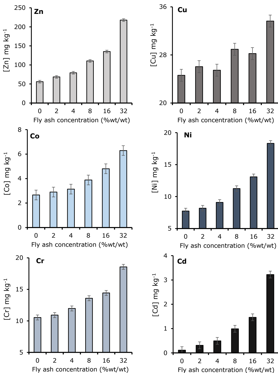
Figure 6-5: Effect of UK fly ash application on total soil concentration of the potentially toxic elements in woodland and arable soils (ash as a single factor in ANOVA). Individual error bars are based on the pooled variance estimate from the ANOVA with 24 degrees of freedom. LSD for Zn= 10.24, Cu= 2.93, Co= 0.68, Ni= 1.27, Cr= 1.16 and Cd= 0.411
