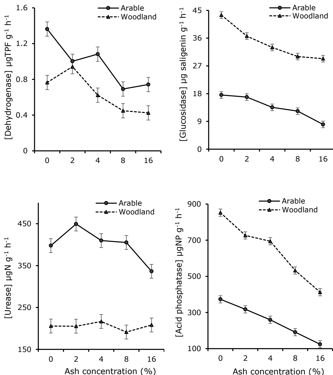
Figure 5-5: Enzymatic activities in soils amended with the Tanzanian ash (TZ1) under wheat plants after 50 days. LSD for dehydrogenase=0.232, glucosidase=3.1, urease=47.96, and acid phosphatase=57.89. The individual error bars are based on the pooled variance estimate from the ANOVA with 30 degrees of freedom. Please note the scale differences on the Y-axes.
