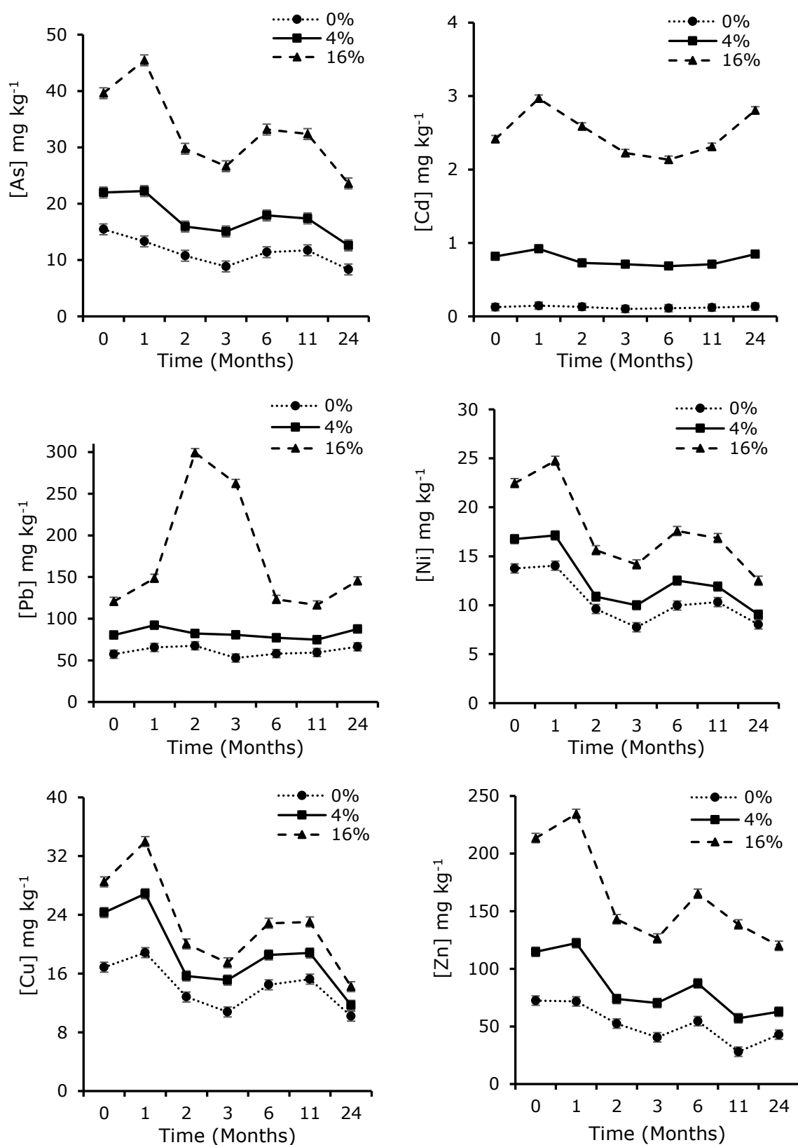
Figure 4-5: Ash induced changes on total PTE concentrations (As, Cd, Pb, Ni, Cu and Zn) following soil incubation for 24 months. Individual error bars are based on the pooled variance estimate from the ANOVA with 60 degrees of freedom. LSD for As=2.722, Cd =0.1382, Pb=13.85, Ni=1.32, Cu=1.922 and Zn=11.48.
