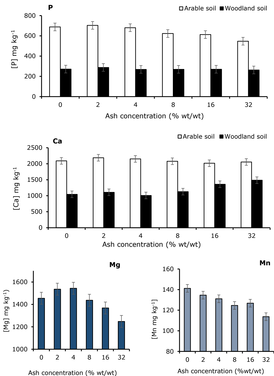
Figure 6-12: Effect of coal ash application on total nutrients concentration (mg kg -1 ) in woodland and arable soils. Individual error bars are based on the pooled variance estimate from the ANOVA with 33 degrees of freedom. LSD (for interaction terms) for P = 59.19 and Ca = 297.3; LSD (ash concentration as a single factor) for Mg = 153.7 and Mn = 10.71.
