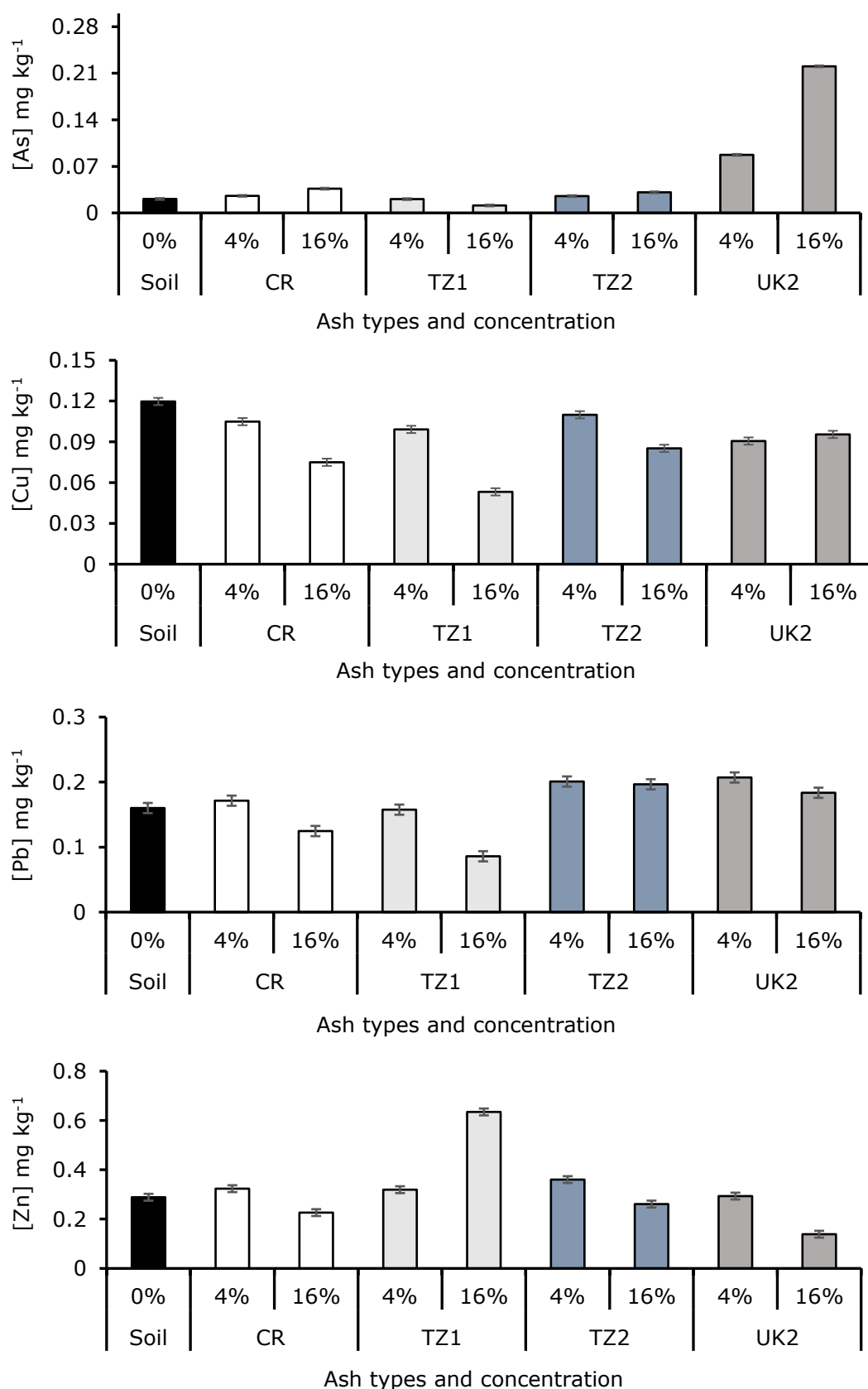
Figure 4-21: The effect of different ashes on water extractable PTEs following a short-term soil incubation. Individual error bars are based on the pooled variance estimate from the ANOVA with 27 degrees of freedom. LSD for As= 0.004, Cu= 0.008, Pb 0.023= and Zn= 0.040. CR, TZ1, TZ2 and UK2 are the Czech Republic, Tanzania batch 1, Tanzania batch 2 and UK batch 2 ash, respectively.
