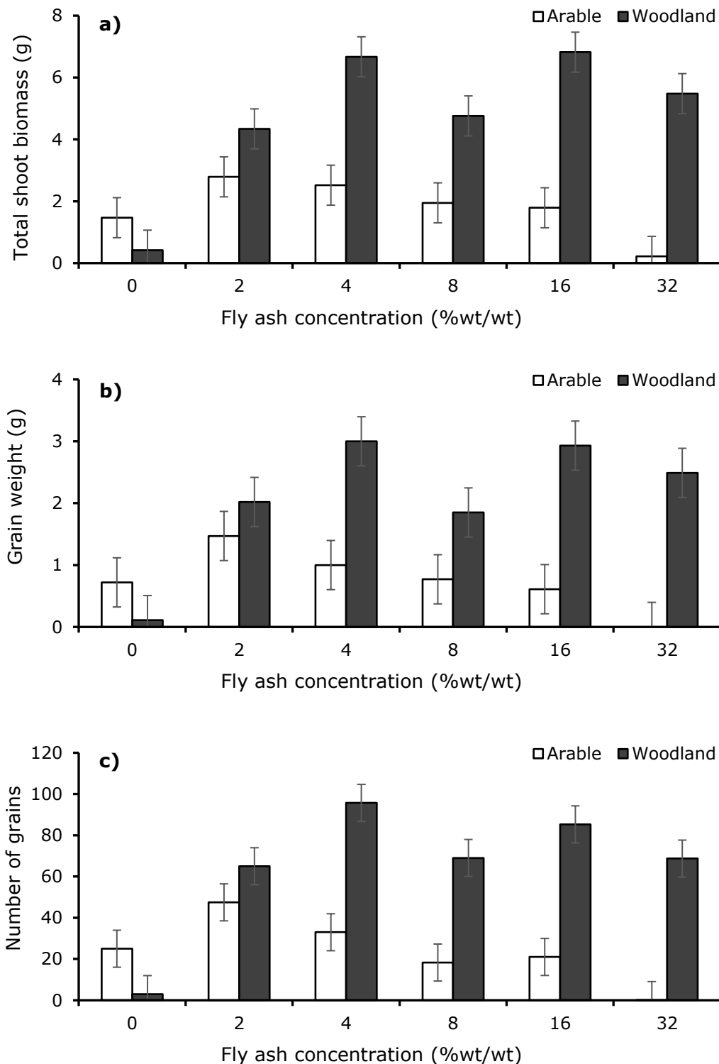
Figure 6-3: Effect of UK ash application on a) shoot biomass, b) grain weight and c) grain number of wheat grown in woodland and arable soils. Individual error bars are based on the pooled variance estimate from the ANOVA with 23 (for total shoot biomass), 19 (for grain number) and 18 (for grain weight) degrees of freedom. LSD for total shoot biomass = 1.89, grain weight = 1.18 and grain number = 26.56.
