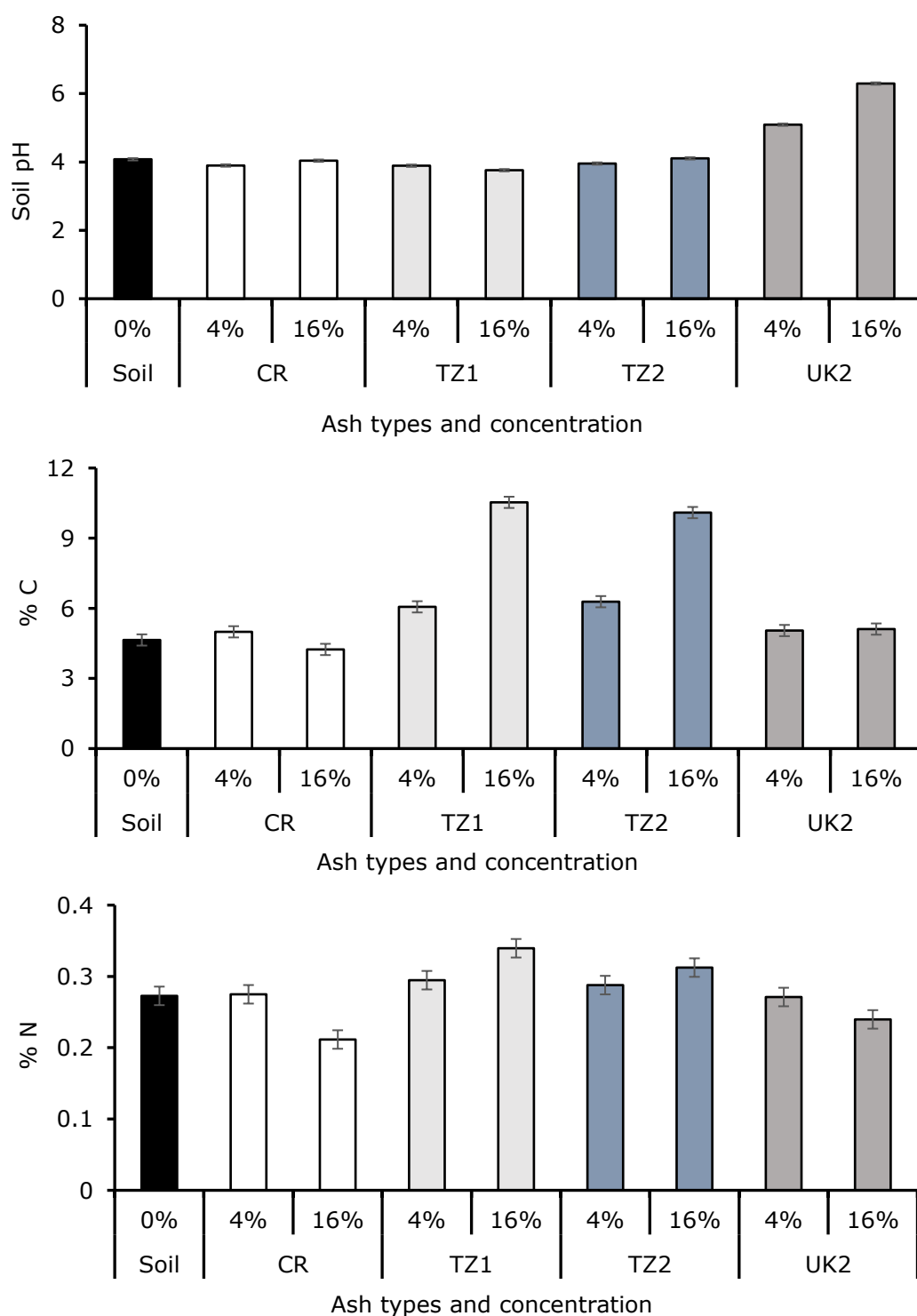
Figure 4-15: The effect of different ashes on soil pH, total C and N following a short-term soil incubation. Individual error bars are based on the pooled variance estimate from the ANOVA with 27 degrees of freedom. LSD for pH=0.099, C=0.698, and N=0.0377. CR, TZ1, TZ2 and UK2 are the Czech Republic, Tanzania batch 1, Tanzania batch 2 and UK batch 2 ash, respectively.
