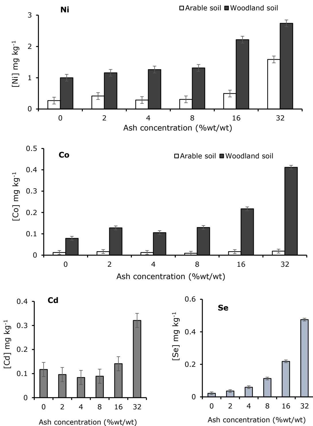
Figure 6-22: Total concentration of PTEs in grains of wheat grown in woodland and arable soil amended with ash. Individual error bars are based on the pooled variance estimate from the ANOVA with 29 degrees of freedom. LSD (for interaction term) for Ni=0.31, Co=0.027, Cd=0.085 and Se=0.025.
