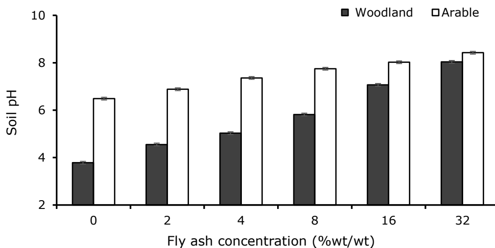
Figure 6-1: The effect of UK fly ash application on pH of woodland and arable soils after harvesting. Individual error bars are based on the pooled variance estimate from the ANOVA with 24 degrees of freedom. LSD=0.17
