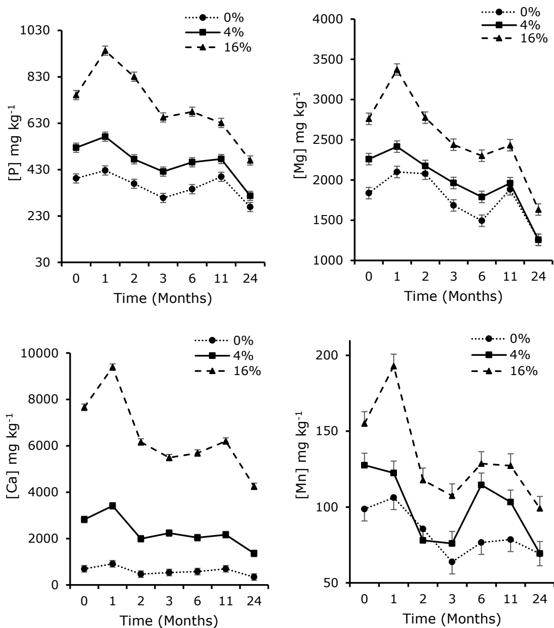
Figure 4-4: Ash induced changes on total soil nutrient concentrations (P, Mg, Ca and Mn) following soil incubation for 24 months. Individual error bars are based on the pooled variance estimate from the ANOVA with 60 degrees of freedom. LSD for P=55.92, Mg= 201.9, Ca=400.1 and Mn=22.3. Please note the scale differences on the Y-axis.
