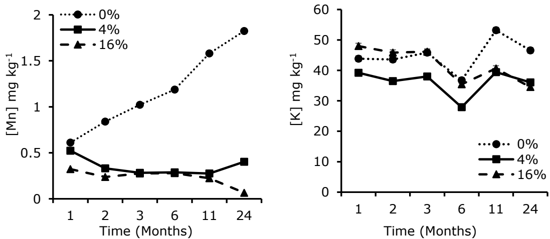
Figure 4-12: Ash induced changes in water extractable nutrient concentrations (K and Mn) following soil incubation for 24 months. Individual error bars are based on the pooled variance estimate from the ANOVA with 54 degrees of freedom. LSD for K= 2.632 and Mn= 0.1453
