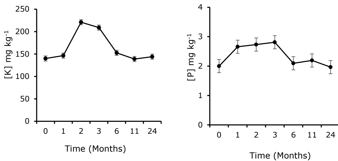
Figure 4-8: Ash induced changes in exchangeable nutrient concentrations (K and P) following soil incubation for 24 months. Data for ash concentrations are pooled. Individual error bars are based on the pooled variance estimate from the ANOVA with 63 degrees of freedom. LSD for K=16.27 and P=0.63
