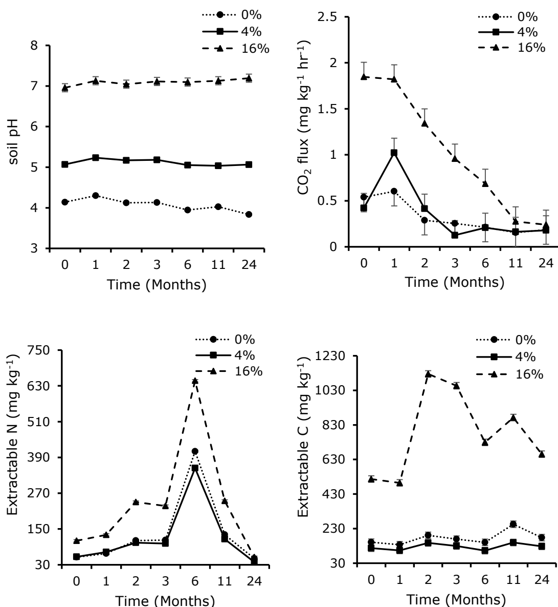
Figure 4-2: Ash induced changes on soil pH, soil respiration ( \text{CO}_2 flux), extractable N and C during soil incubation for 24 months. Individual error bars are based on the pooled variance estimate from the ANOVA with 60 (pH), 51 (extractable N) and 54 (for \text{CO}_2 flux and extractable C) degrees of freedom. LSD for pH=0.057, \text{CO}_2 flux=0.449, extractable N=10.52 and extractable C=53.24. Please note the scale differences on the Y-axes.
