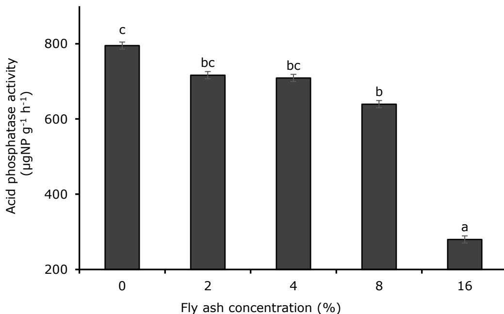
Figure 5-3: Acid phosphatase in woodland soil amended with different concentrations of the UK1 fly ash. Columns with the same letters are not significantly different according to Tukey's multiple comparison test, p < 0.001 .
