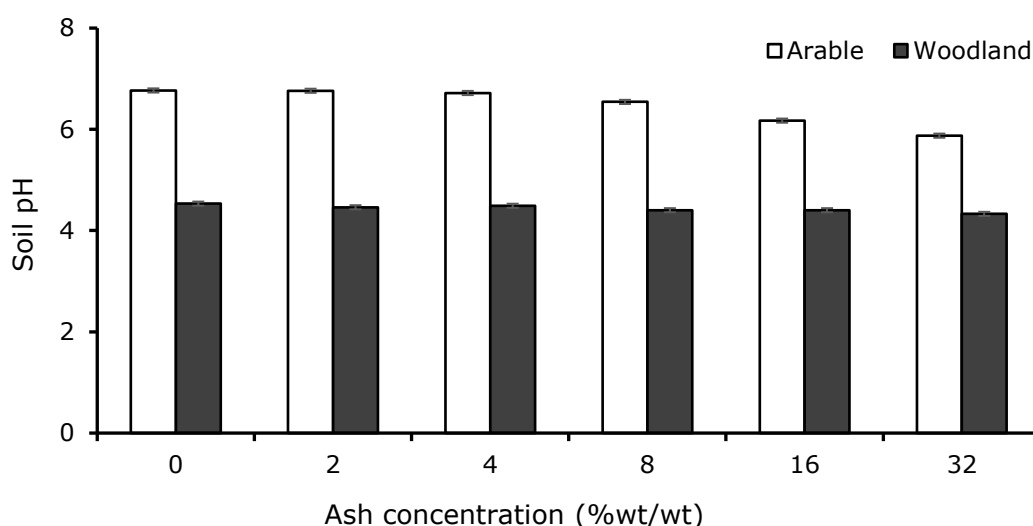
Figure 6-9: The effect of coal ash application on soil pH after harvesting, p < 0.001 (ash concentration \times soil type interaction), LSD = 0.11 .
