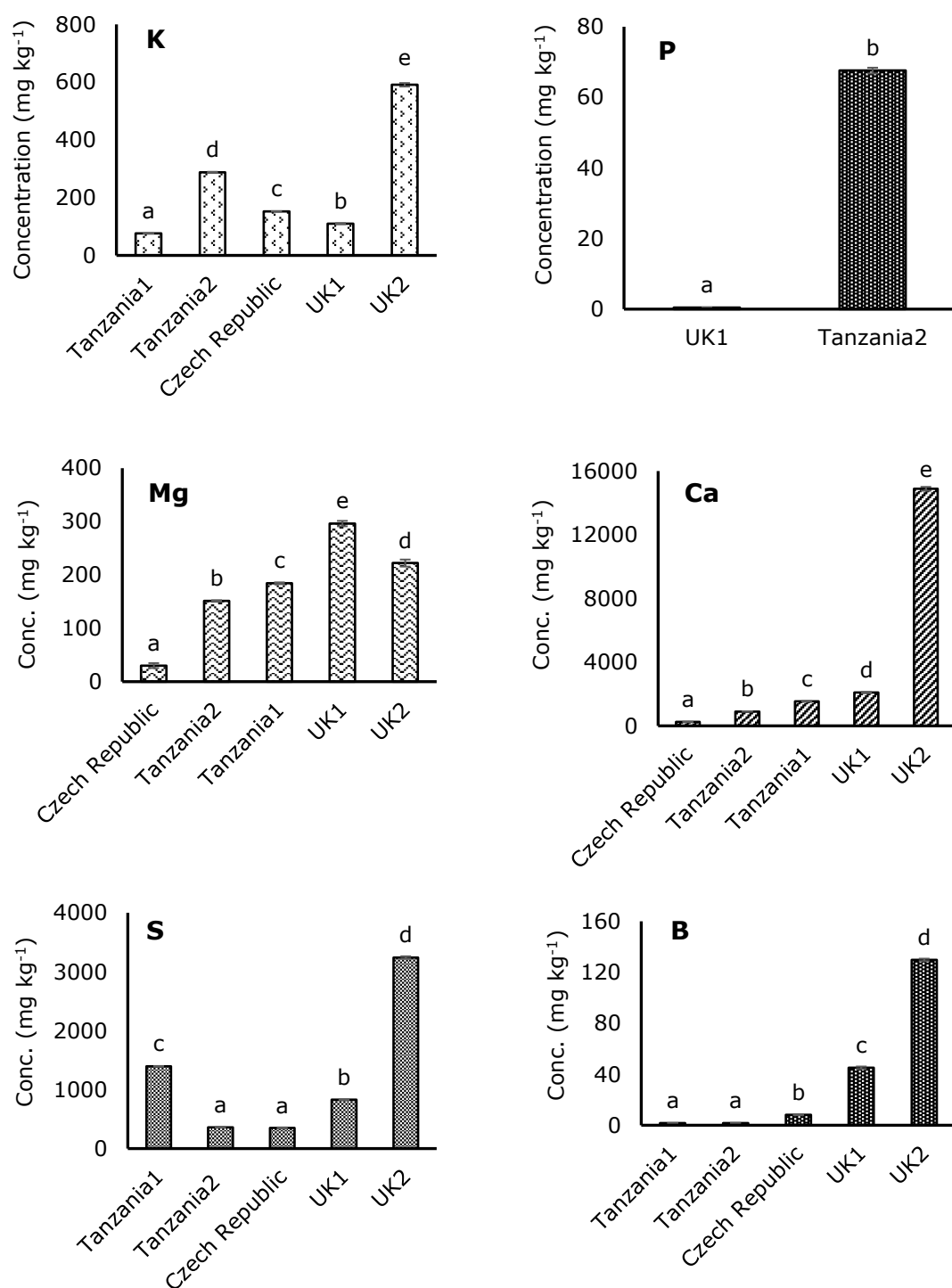
Figure 3-4: Exchangeable concentrations (mg kg -1 ) of nutrients in ash from UK, Czech Republic and Tanzania. Values given are means of four replicates \pm standard errors. Columns similarly superscripted are not significantly different (Tukey's Test). P content in Tanzania1, UK2 and Czech Republic ashes is not presented because it was below detection limit according to the standards during ICP analysis.
