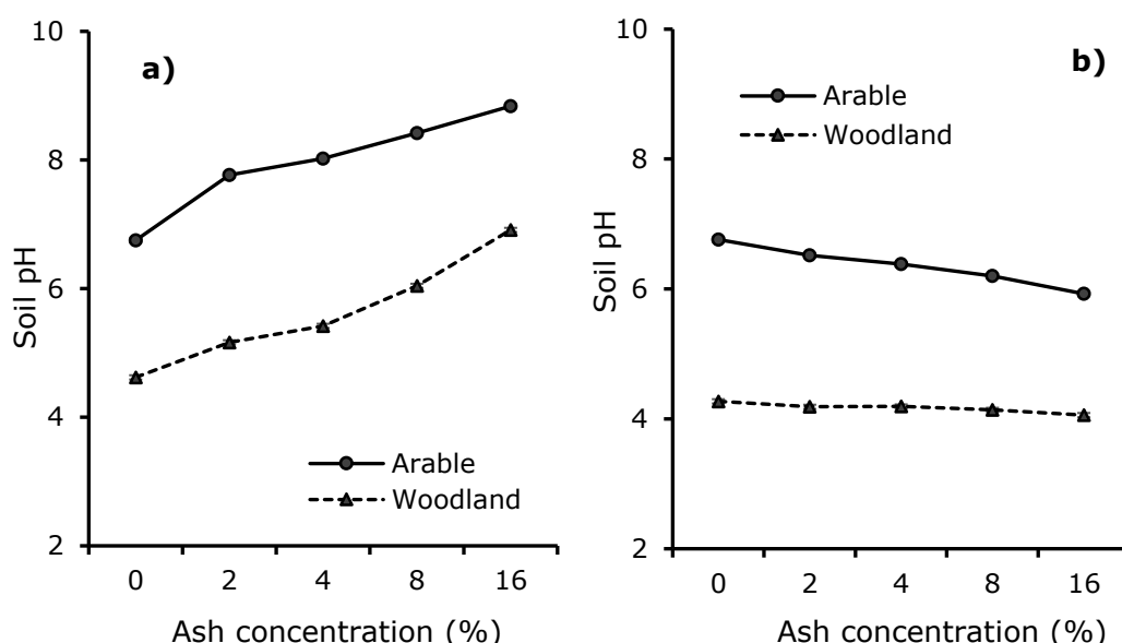
Figure 5-1: Effect of ash application on soil pH. a) = The soil treated with the UK1 ash, LSD=0.095 , SE=0.033 and b) = the soil treated with Tanzanian ash, LSD=0.068 , SE=0.024 . The individual error bars are based on the pooled variance estimate from the ANOVA with 30 degrees of freedom.
