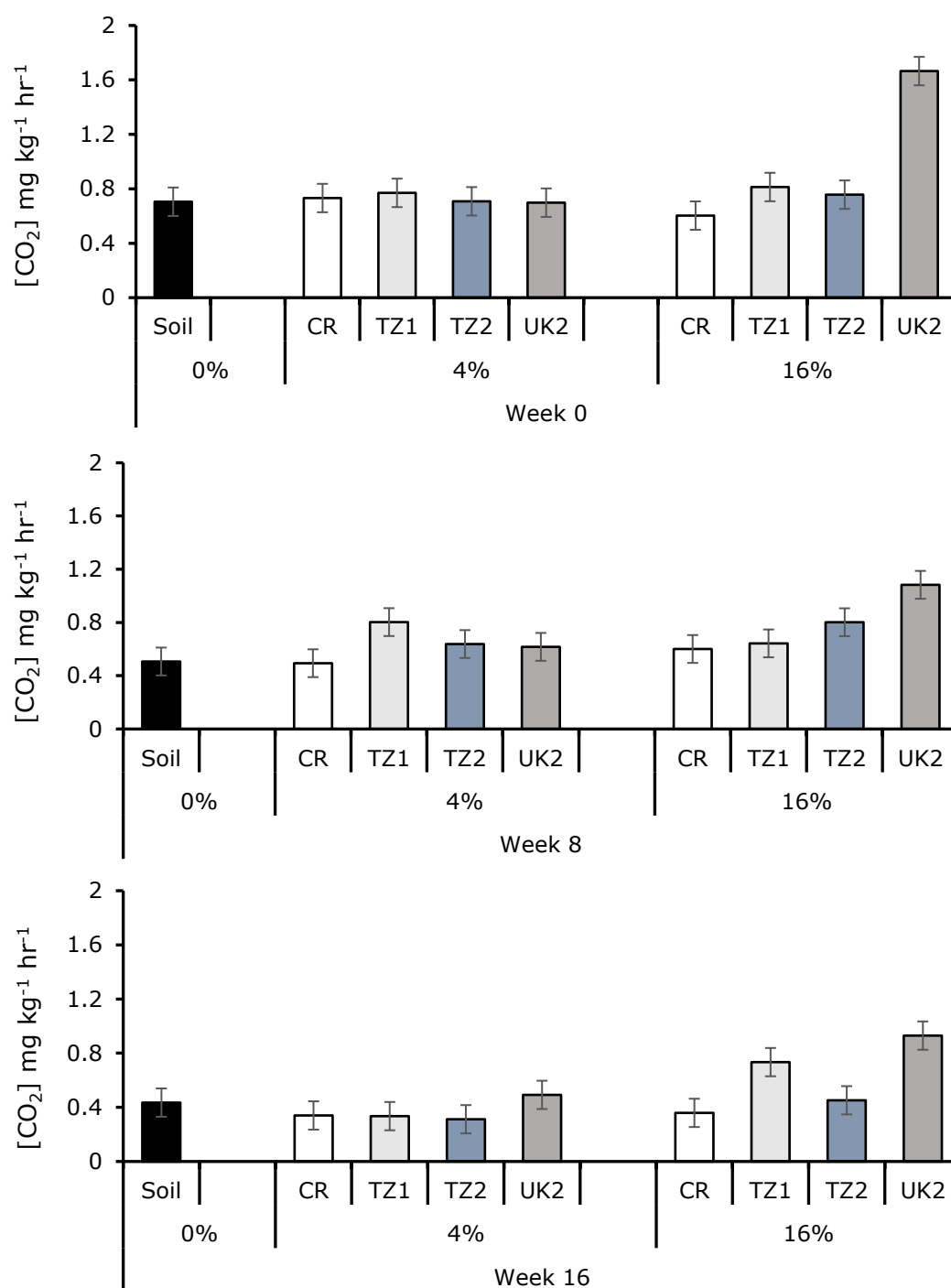
Figure 4-14: The effect of different ashes on soil respiration (CO 2 evolution rate) during soil incubation for 16 weeks. Individual error bars are based on the pooled variance estimate from the ANOVA with 50 degrees of freedom. LSD for CO 2 flux = 0.3642. CR, TZ1, TZ2 and UK2 are the Czech Republic, Tanzania batch 1, Tanzania batch 2 and UK batch 2 ash, respectively.
