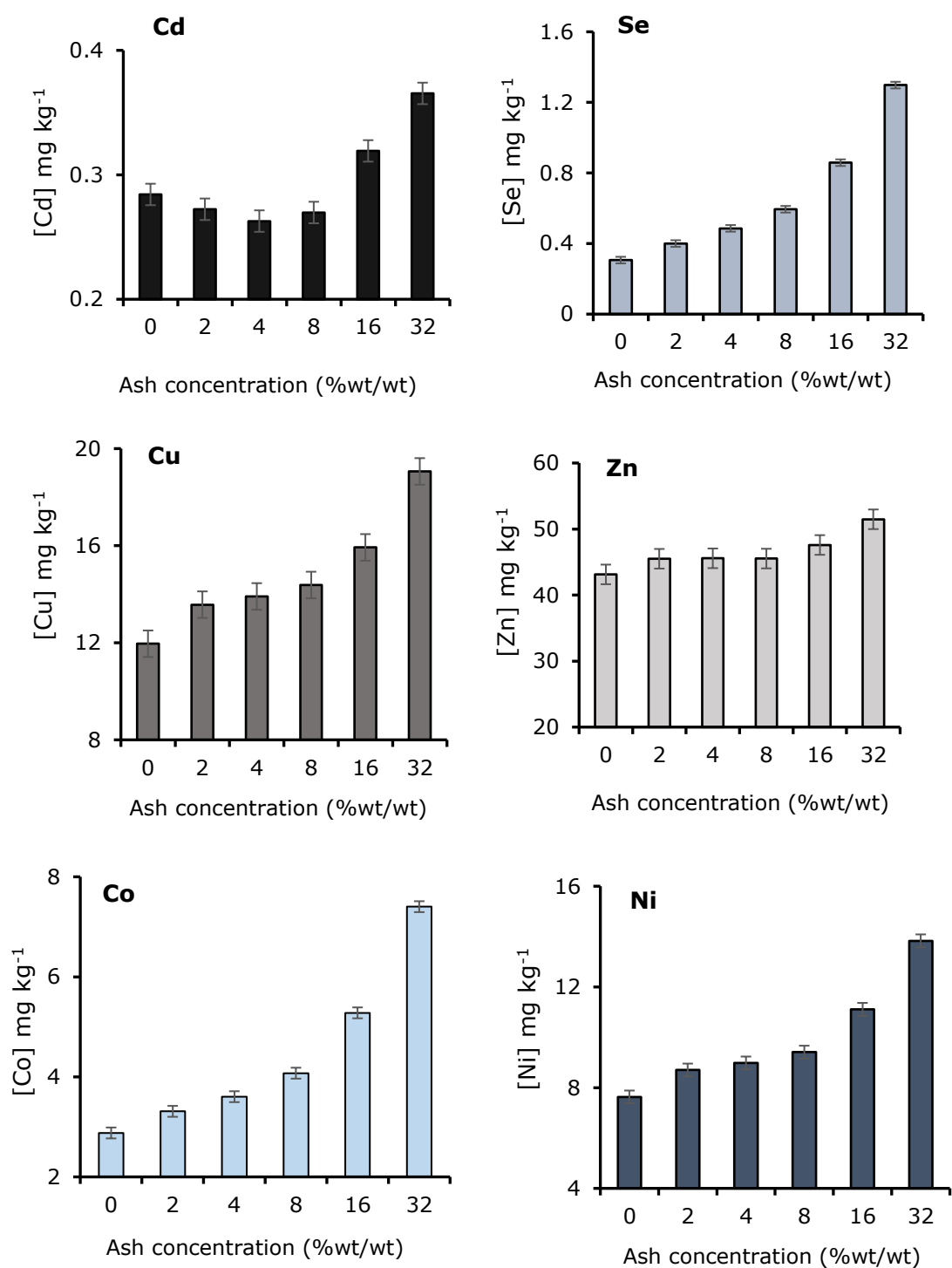
Figure 6-13: Effect of coal ash application on total soil concentration (mg kg -1 ) of the potentially toxic elements in woodland and arable soils (ash as a single factor, Table 10-11). Individual error bars are based on the pooled variance estimate from the ANOVA with 33 degrees of freedom. LSD for Cd=0.025, Se=0.054, Cu=1.57, Zn=4.28, Co=0.31 and Ni=0.74. Data are pooled across both soil types.
