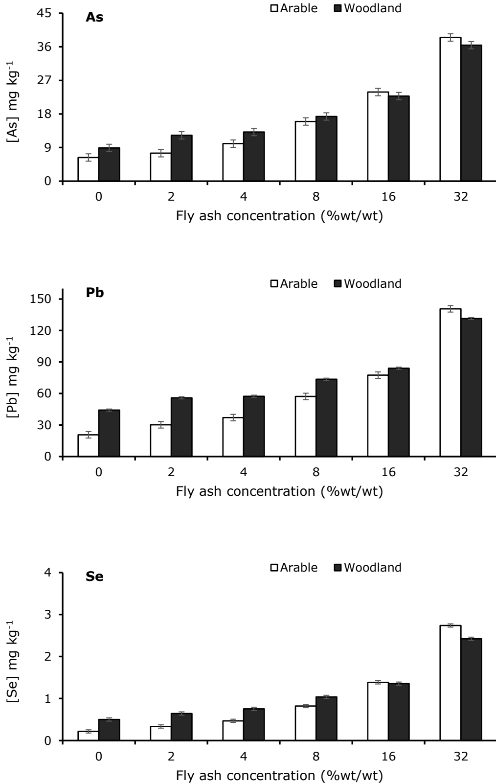
Figure 6-6: Effect of UK fly ash application on total soil concentration of the potentially toxic elements, As, Pb and Se in woodland and arable soils (ash concentration \times soil type interaction). Individual error bars are based on the pooled variance estimate from the ANOVA with 24 degrees of freedom. LSD for As=2.89, Pb=9.06 and Se=0.11.
