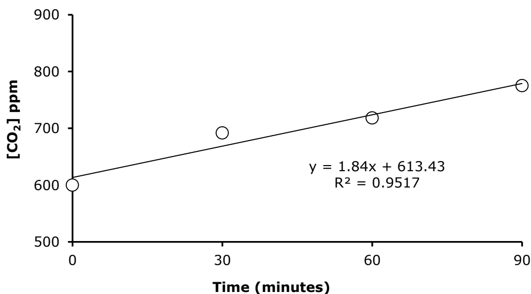
Figure 4-1: An example of the rate of CO 2 evolution with time from soil amended with fly ash.
