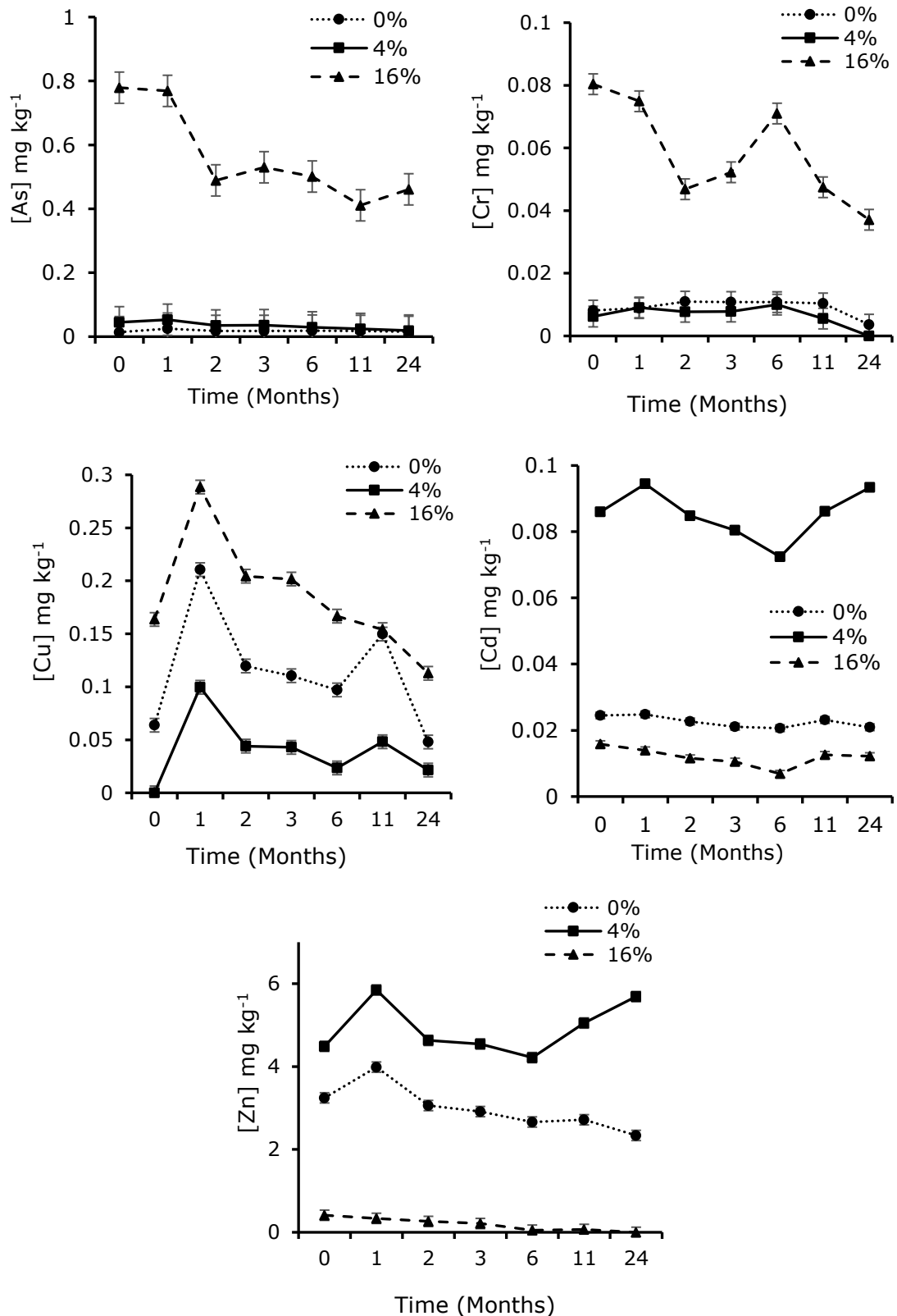
Figure 4-9: Ash induced changes in exchangeable PTE concentrations (As, Cr, Cu, Cd and Zn) following soil incubation for 24 months. Individual error bars are based on the pooled variance estimate from the ANOVA with 63 degrees of freedom. LSD for As=0.1383, Cr= 0.009, Cu=0.018, Cd=0.0029, and Zn=0.3489
