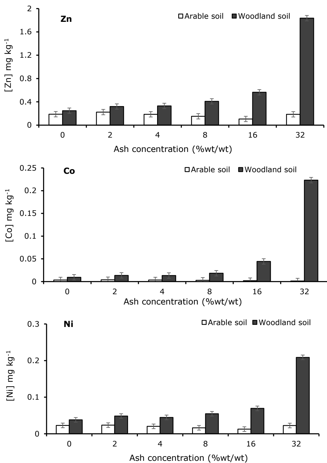
Figure 6-18: Effect of coal ash application on water extractable concentration of the potentially toxic elements in woodland and arable soils. Individual error bars are based on the pooled variance estimate from the ANOVA with 33 degrees of freedom. LSD for Zn=0.13, Co= 0.017 and Ni= 0.018.
