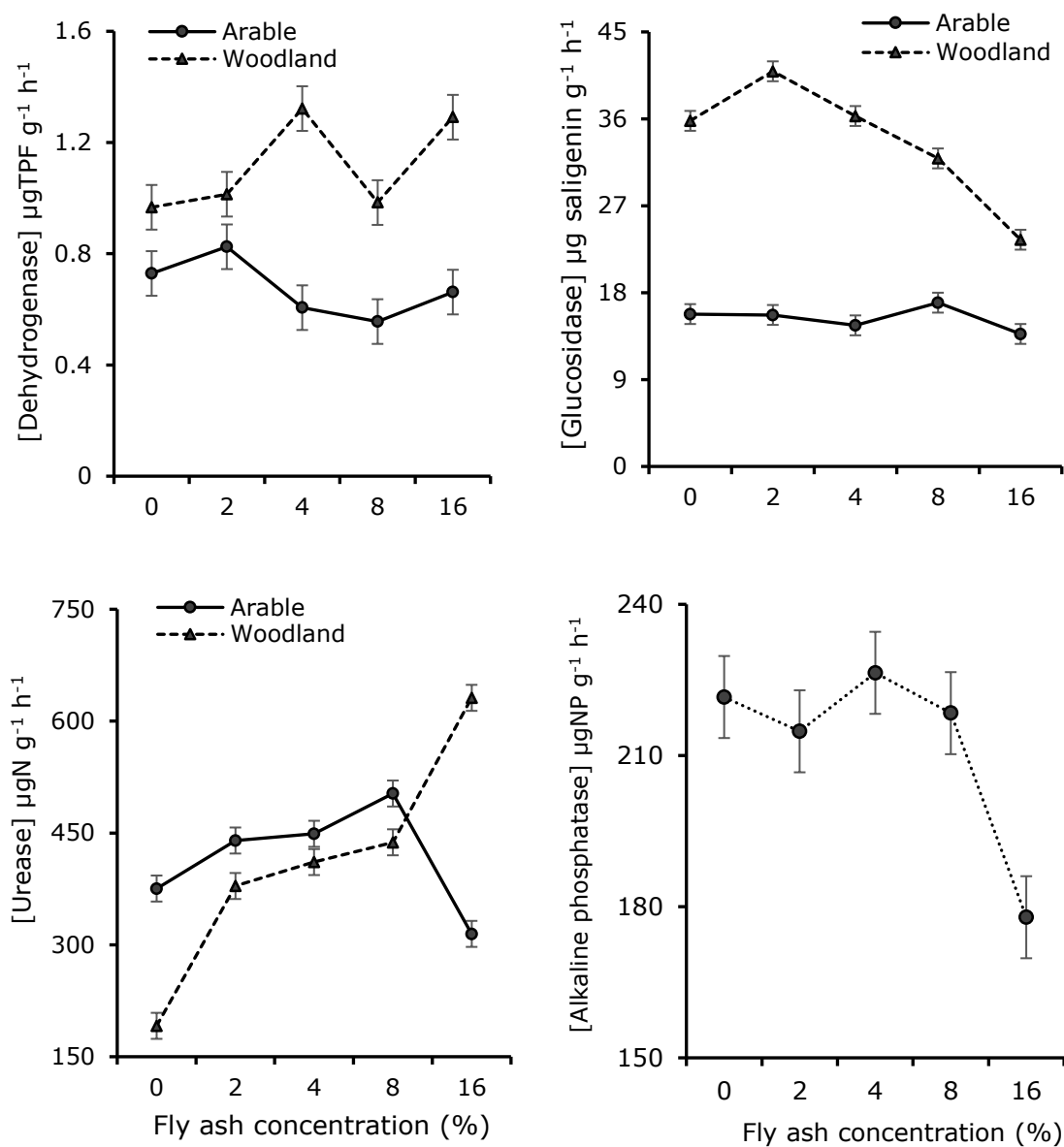
Figure 5-2: Enzyme activities in UK1 fly ash amended soils, under wheat plants for 50 days. LSD for dehydrogenase=0.261, glucosidase=2.97, urease=50.4, and alkaline phosphatase=23.52. The individual error bars are based on the pooled variance estimate from the ANOVA with 30 degrees of freedom. Please note the scale differences on the Y-axes. For alkaline phosphatase, data are means pooled across the woodland and arable soils.
