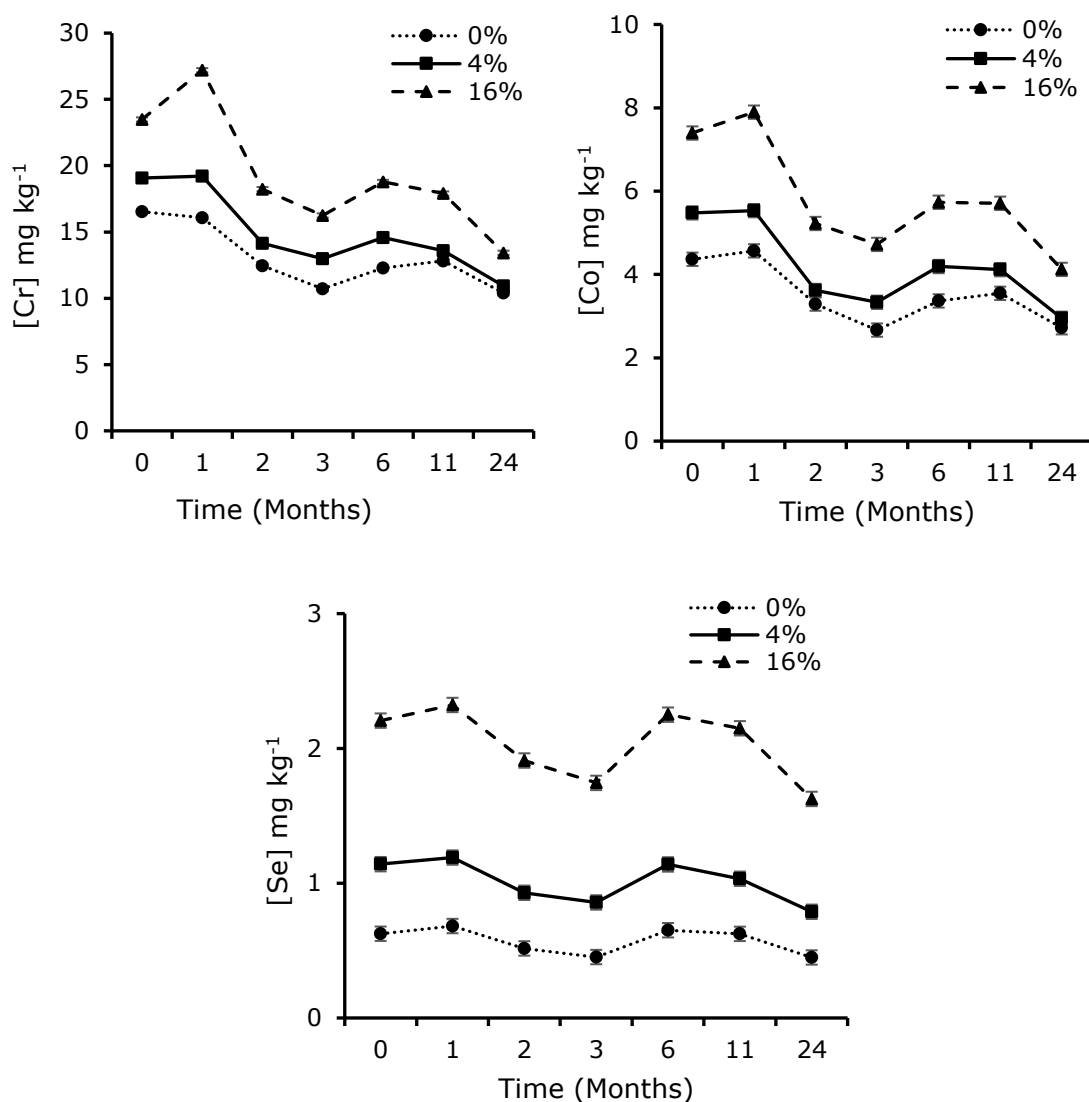
Figure 4-6: Ash induced changes on total PTE concentrations (Cr, Co and Se) following soil incubation for 24 months. Individual error bars are based on the pooled variance estimate from the ANOVA with 60 degrees of freedom. LSD for Cr=1.647, Co=0.4524, and Se=0.1512
