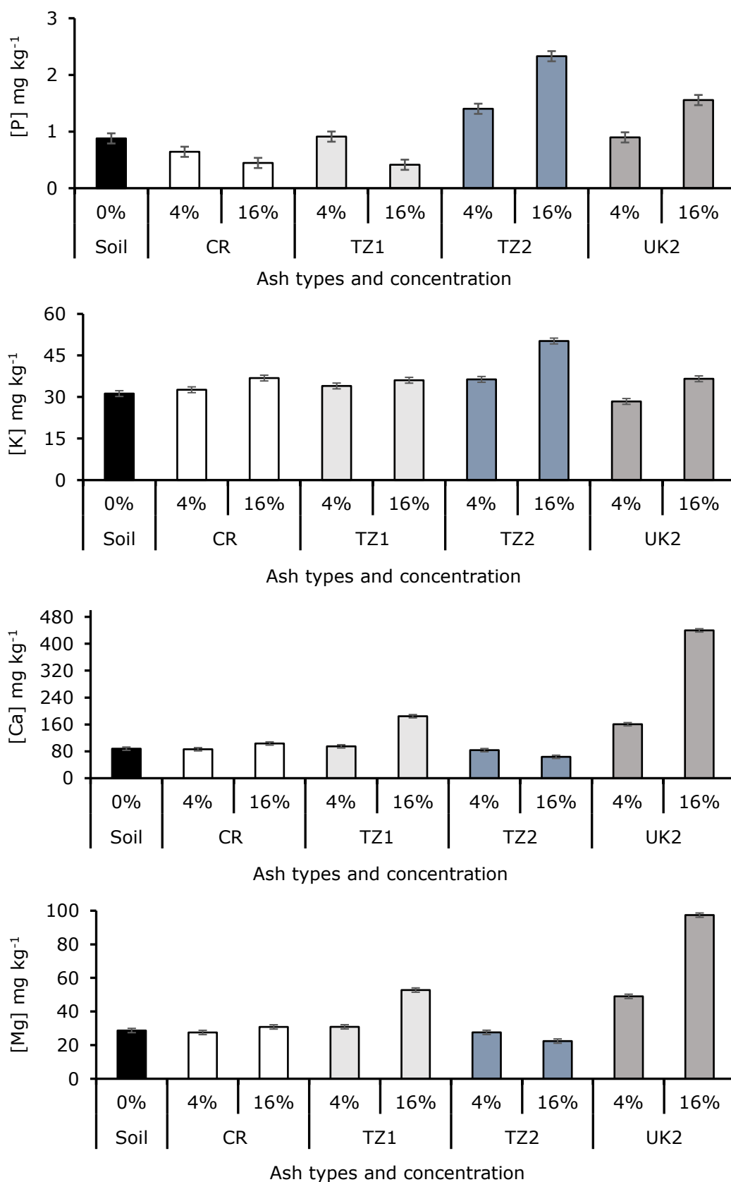
Figure 4-19: The effect of different ashes on water extractable nutrients following a short-term soil incubation. Individual error bars are based on the pooled variance estimate from the ANOVA with 27 degrees of freedom. LSD for P= 0.261, K= 3.032, Ca= 14 and Mg=3.721. CR, TZ1, TZ2 and UK2 are the Czech Republic, Tanzania batch 1, Tanzania batch 2 and UK batch 2 ash, respectively.
