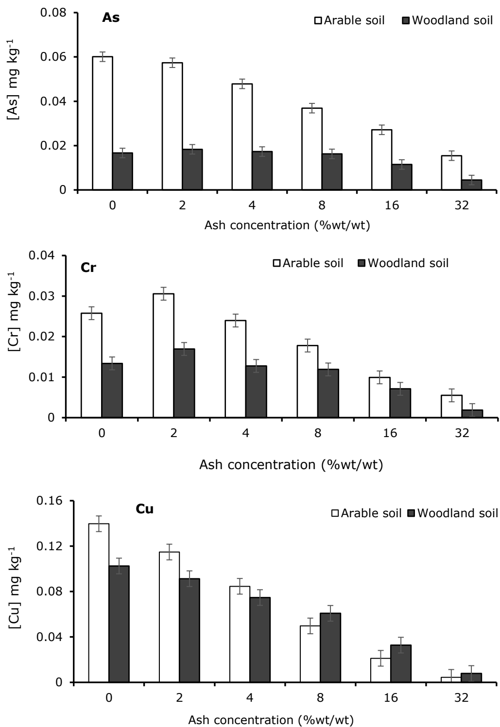
Figure 6-16: Effect of coal ash application on water extractable concentration of the potentially toxic elements in woodland and arable soils. Individual error bars are based on the pooled variance estimate from the ANOVA with 33 degrees of freedom. LSD for As= 0.006, Cr= 0.005, Cu= 0.020. Please take note of scale differences on Y axes. See Table 6-12 for corresponding ANOVA output.
