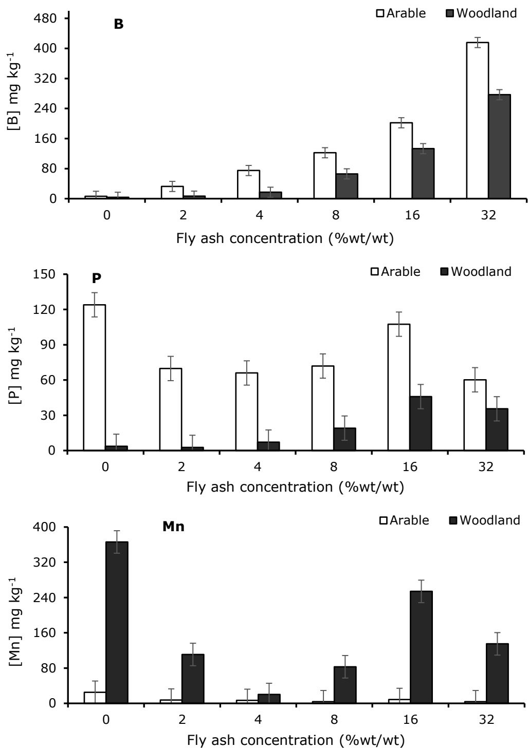
Figure 6-7: The effect of fly ash on water extractable B, P and Mn in woodland and arable soils. Individual error bars are based on the pooled variance estimate from the ANOVA with 22 degrees of freedom. LSD for B= 39.59, P= 30.32 and Mn= 74.86. Please take note of scale differences on the Y axes.
