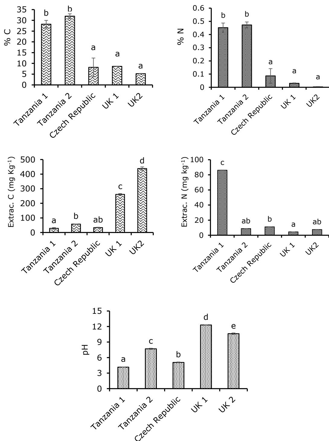
Figure 3-1: Chemical properties of coal ash samples collected from UK, the Czech Republic and Tanzania. Values given are means of four replicates \pm standard errors. Total extractable C and N were extracted by 0.5M K_2SO_4 1:5 ratio. Columns similarly superscripted are not significantly different (Tukey's Test). Total extractable C = sum of total extractable organic carbon (TOC) and inorganic carbon (IC).
