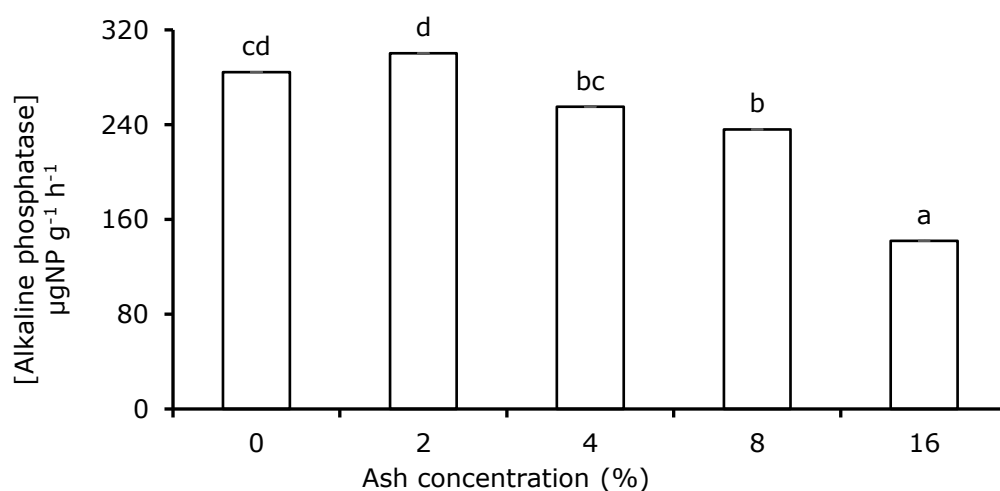
Figure 5-6: Alkaline phosphatase in the arable soil amended with different concentrations of the Tanzanian ash. Columns with the same letters are not significantly different according to Tukey's multiple comparison test, p < 0.001 , F_{4, 15} = 42.41
