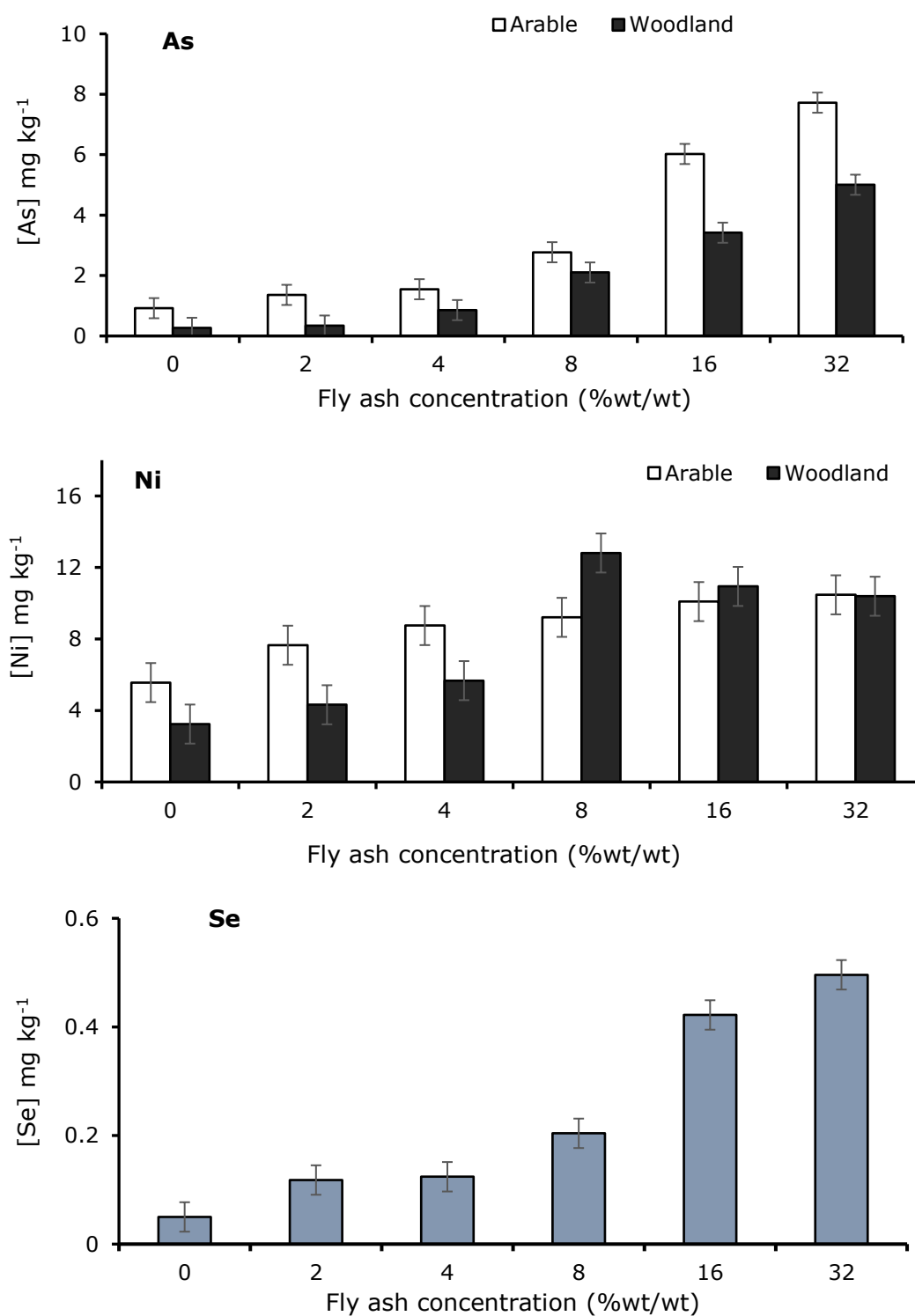
Figure 6-8: Effect of fly ash application on water extractable concentration of the potentially toxic elements As, Ni and Se in woodland and arable soils. Individual error bars are based on the pooled variance estimate from the ANOVA with 22 degrees of freedom. LSD for As= 0.98, Ni= 3.20, Se= 0.080. Please take note on scale differences in Y axis. Data for Se are pooled means for both soil types because ash concentration was significant as a single factor (see Table 6-5).
