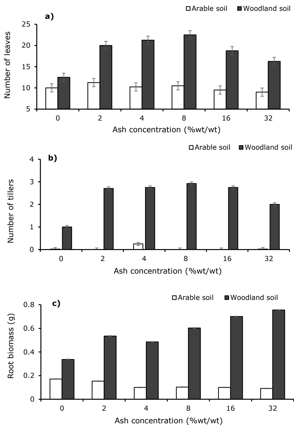
Figure 6-10: Effect of coal ash application on a) number of leaves, b) number of tillers and c) root biomass of wheat grown in woodland and arable soils. Individual error bars are based on the pooled variance estimate from the ANOVA with 29 degrees of freedom. LSD (for the interaction terms) for number of leaves = 2.85, number of tillers = 0.77, and root biomass = 0.16
