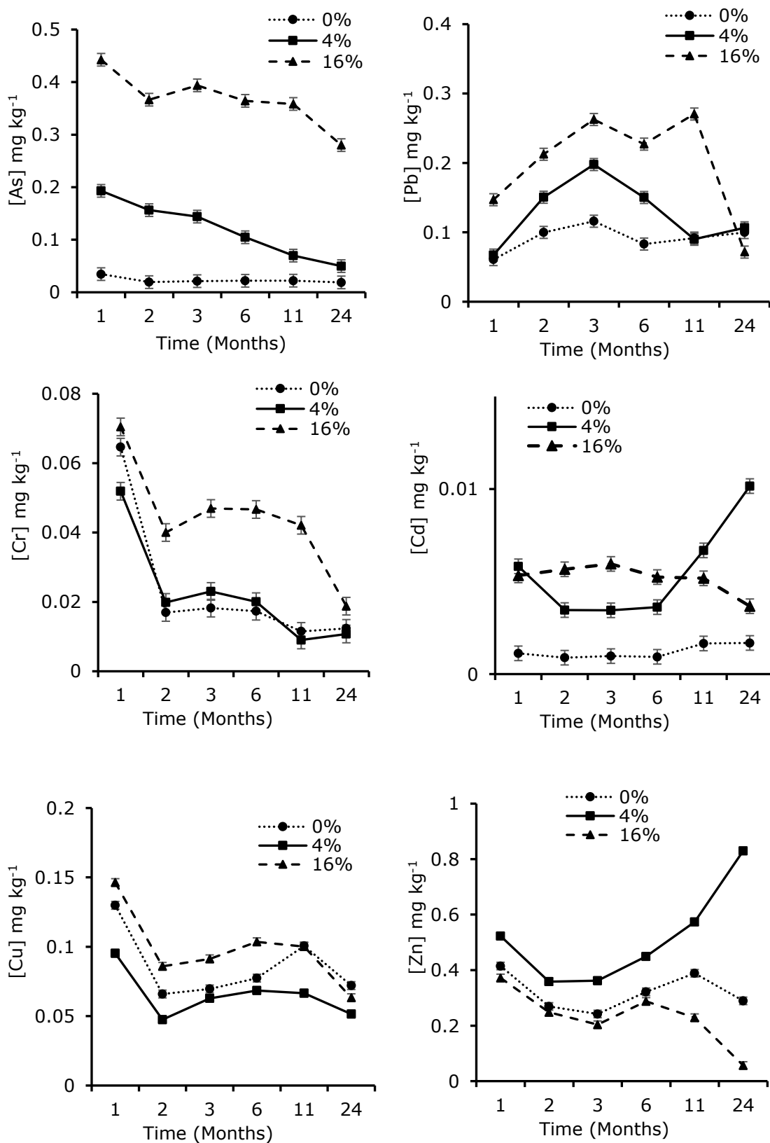
Figure 4-13: Ash induced changes in water extractable PTE concentrations (As, Pb, Cr, Cd, Cu and Zn) following soil incubation for 24 months. Individual error bars are based on the pooled variance estimate from the ANOVA with 54 degrees of freedom. LSD for As=0.034, Pb= 0.0245, Cr= 0.007, Cd=0.001, Cu=0.008, and Zn=0.038
