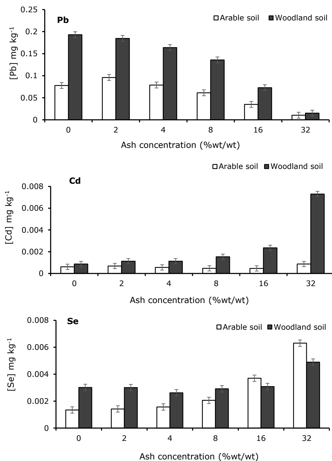
Figure 6-17: Effect of coal ash application on water extractable concentration of the potentially toxic elements in woodland and arable soils. Individual error bars are based on the pooled variance estimate from the ANOVA with 33 degrees of freedom. LSD for Pb= 0.019, Cd= 0.0007, Se=0.0007.
