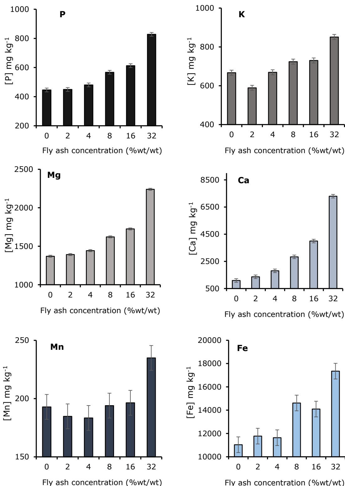
Figure 6-4: Effect of UK fly ash application on total soil nutrient concentrations in woodland and arable soils after harvesting wheat. Data are pooled means from ANOVA (fly ash as a significant single factor). Individual error bars are based on the pooled variance estimate from the ANOVA with 24 (for P, Ca, Mg and Fe), 22 (for K) and 23 (for Mn), degrees of freedom. LSD for P = 38.3, K = 86.7, Mg = 113.0, Ca = 382.6, Mn = 31.2 and Fe = 1962.9
