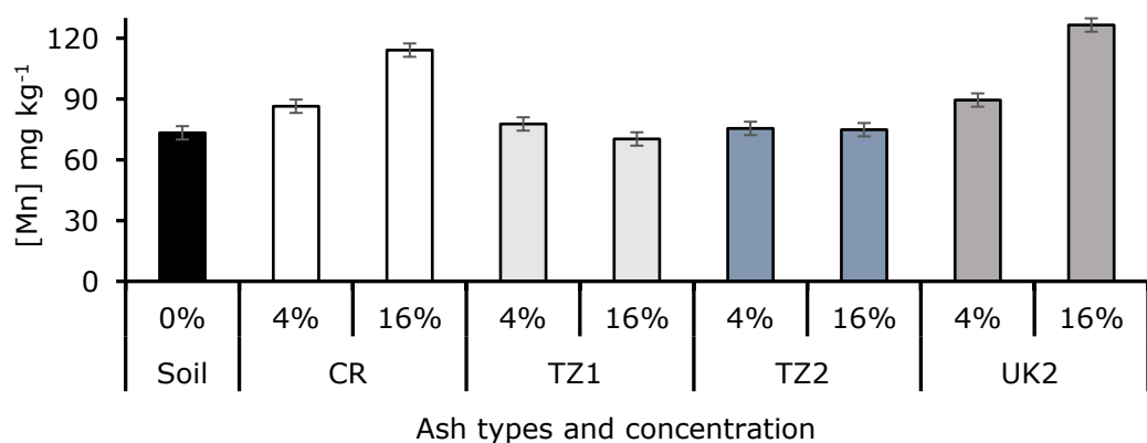
Figure 4-16: The effect of different ashes on total soil nutrients following a short-term soil incubation. Individual error bars are based on the pooled variance estimate from the ANOVA with 27 degrees of freedom. LSD for P= 25.13, Ca= 180.5, Mg= 143.6, and Mn= 9.574. CR, TZ1, TZ2 and UK2 are the Czech Republic, Tanzania batch 1, Tanzania batch 2 and UK batch 2 ash, respectively.
