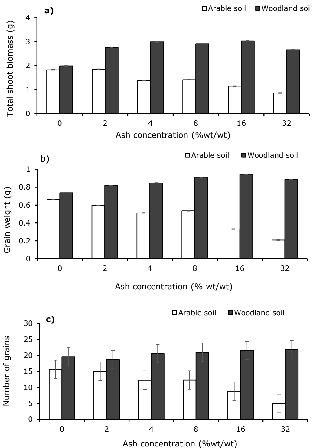
Figure 6-11: Effect of coal ash application on a) shoot biomass, b) grain weight and c) grain number of wheat grown in woodland and arable soils. Individual error bars are based on the pooled variance estimate from the ANOVA with 28 (for grain weight and grain number) and 29 (for total shoot biomass) degrees of freedom. LSD (for the interaction terms) for total shoot biomass = 0.35, grain weight = 0.17, and grain number = 4.92.
