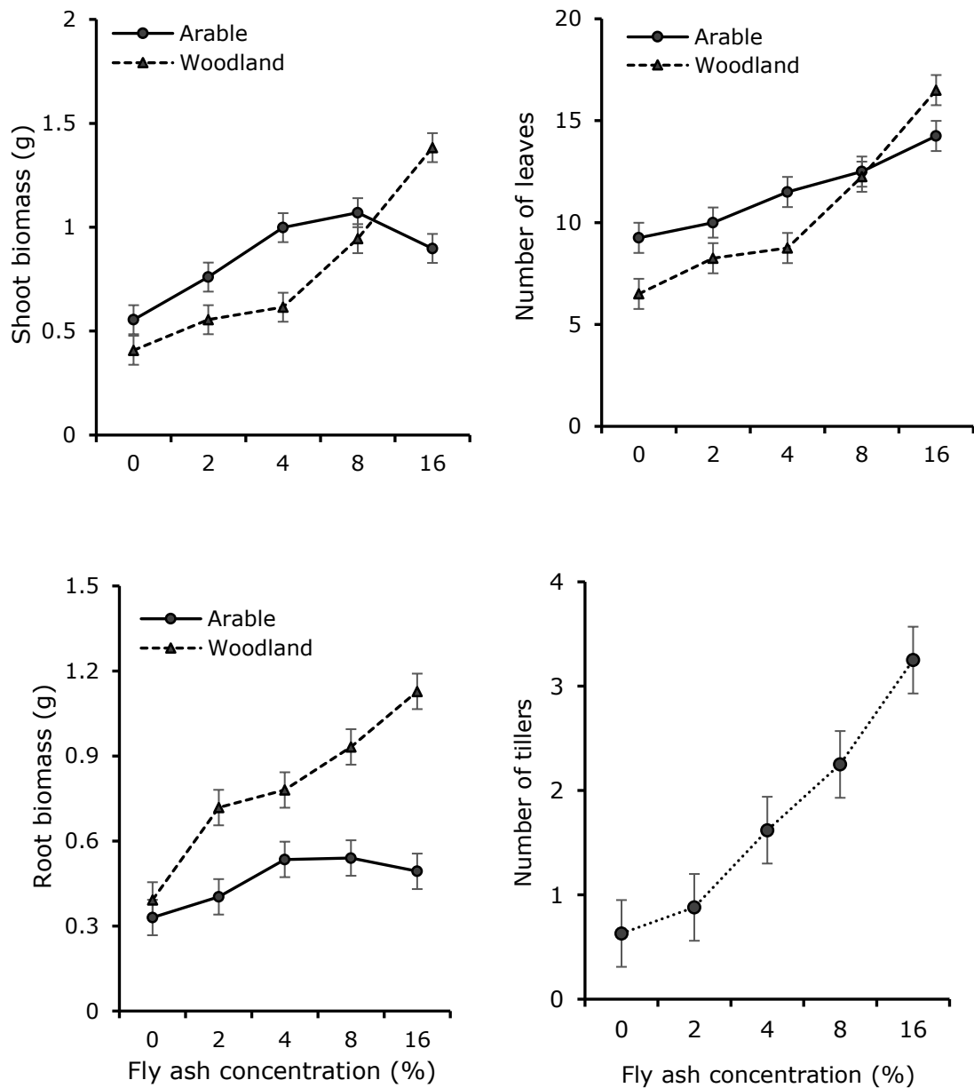
Figure 5-4: The effect of the UK1 fly ash on wheat growth parameters after 50 days. LSD for shoot biomass=0.2017, Number of leaves=2.138, root biomass=0.1807, and number of tillers=0.923. The individual error bars are based on the pooled variance estimate from the ANOVA with 30 degrees of freedom.
