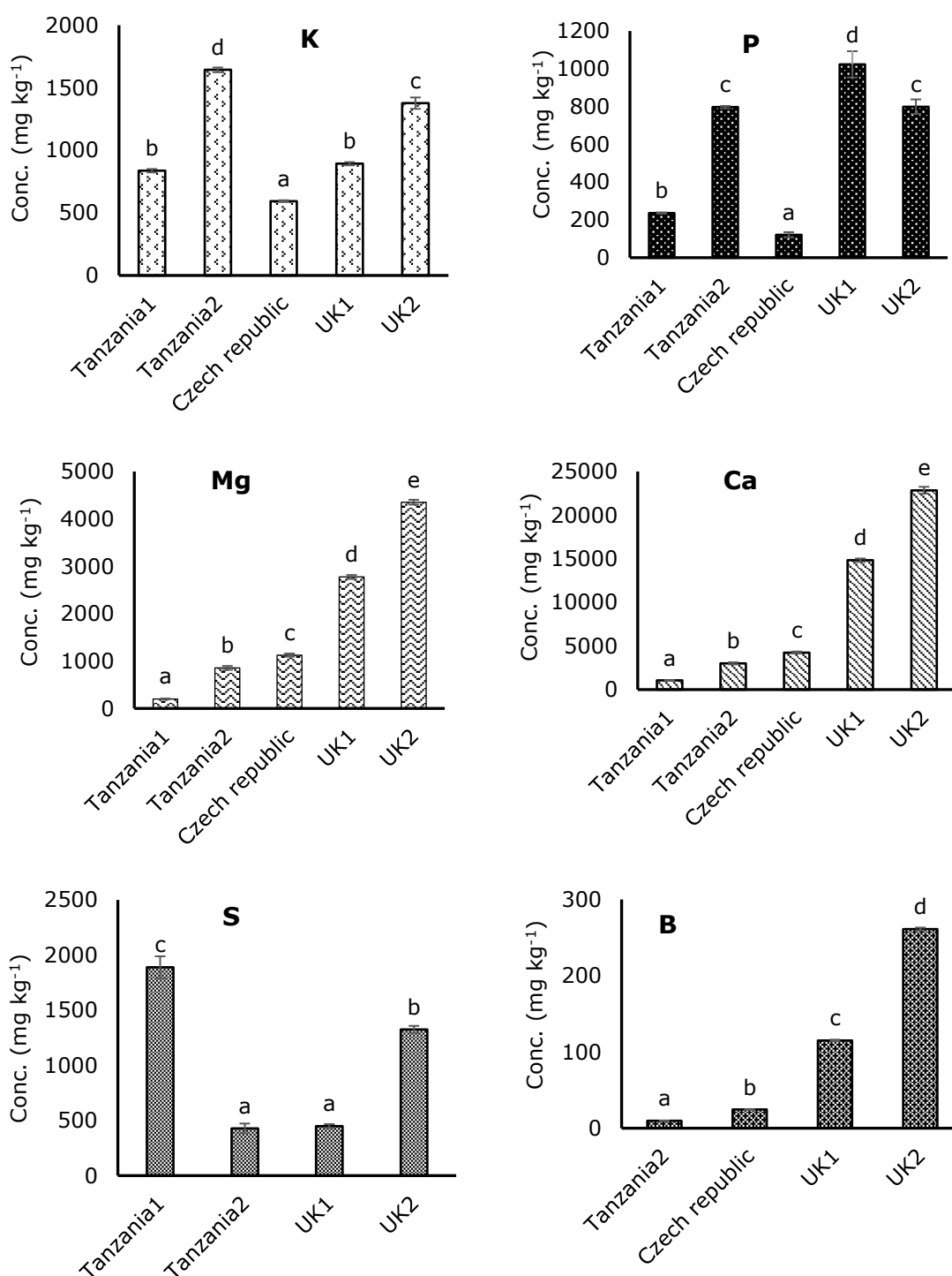
Figure 3-2: Total concentrations (mg kg -1 ) of nutrients in ash from the UK, Czech Republic and Tanzania. Values given are means of four replicates \pm standard errors. Columns similarly superscripted are not significantly different (Tukey's Test). S content in Czech Republic ash and B content in Tanzania1 ash are not presented because they were below the detection limit.
