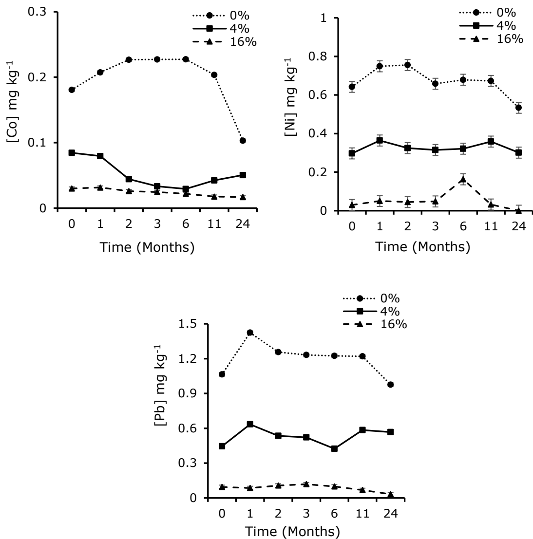
Figure 4-10: Ash induced changes in exchangeable PTE concentrations (Co, Ni, and Pb) following soil incubation for 24 months. Individual error bars are based on the pooled variance estimate from the ANOVA with 63 degrees of freedom. LSD for Co=0.007, Ni=0.081 and Pb=0.044
