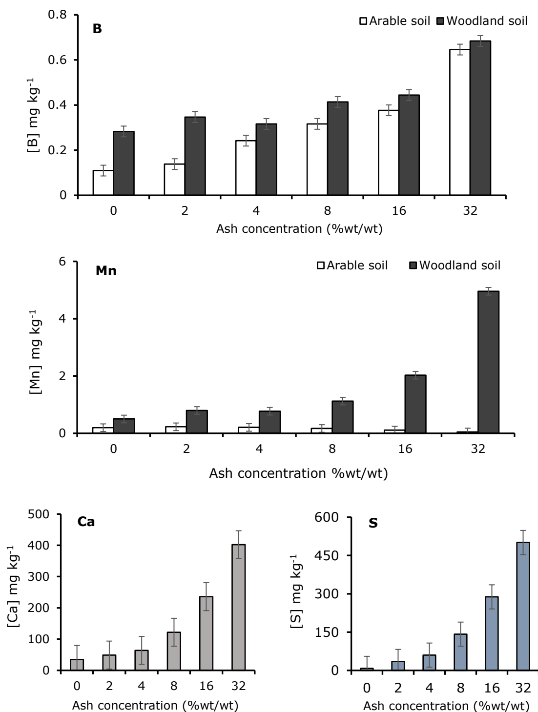
Figure 6-15: Effect of coal ash on water extractable nutrients in woodland and arable soils. Individual error bars are based on the pooled variance estimate from the ANOVA with 33 degrees of freedom. LSD (for interaction terms) for B=0.069 and Mn=0.38; LSD for ash as a single factor for Ca=128.9, and S=136.2. Please take note of scale differences on Y axes.
