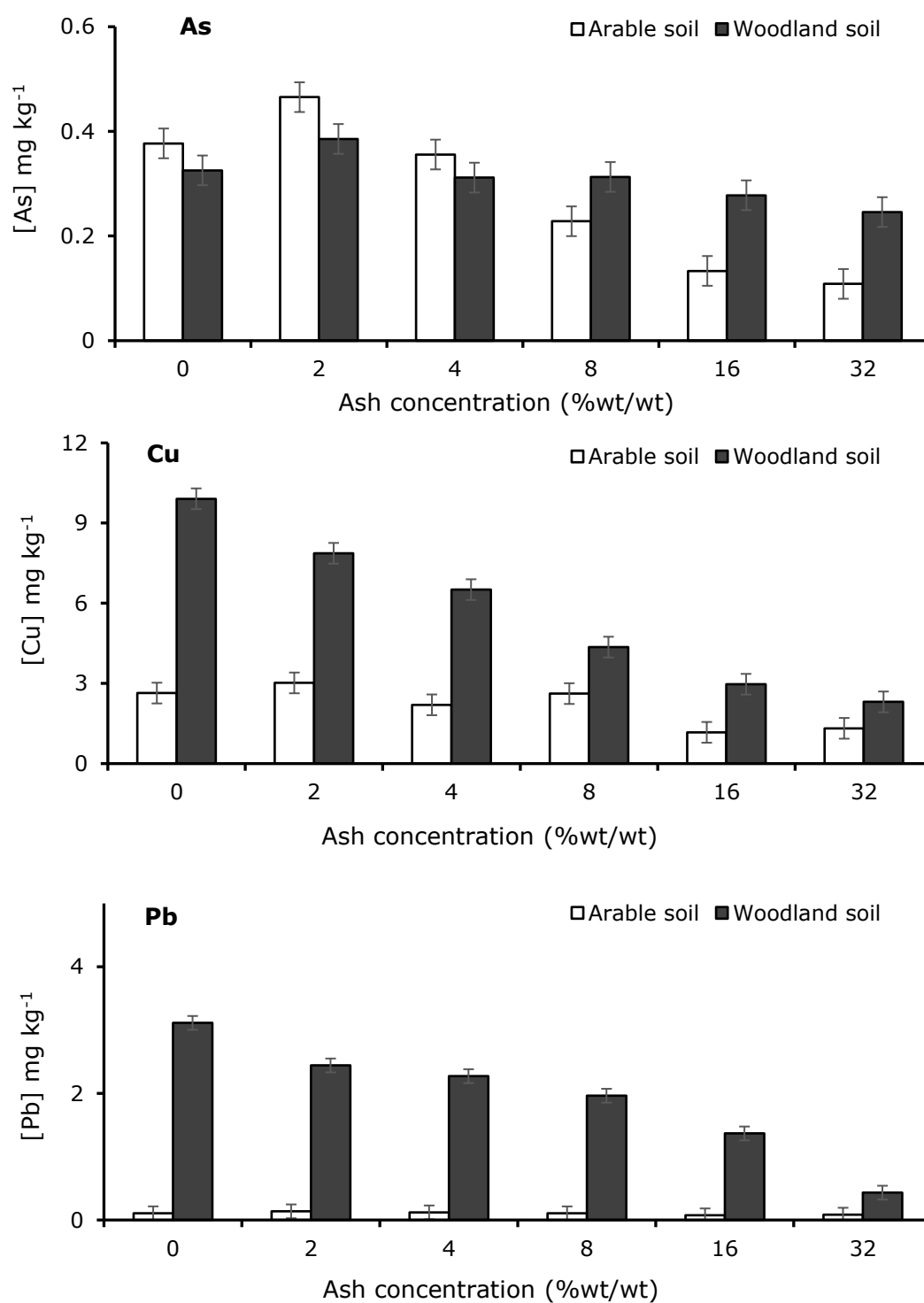
Figure 6-21: Total concentration of PTEs in wheat shoots grown in woodland and arable soil amended with ash. Individual error bars are based on the pooled variance estimate from the ANOVA with 33 degrees of freedom. LSD (for interaction term) for As=0.082, Cu=1.12 and Pb=0.32.
