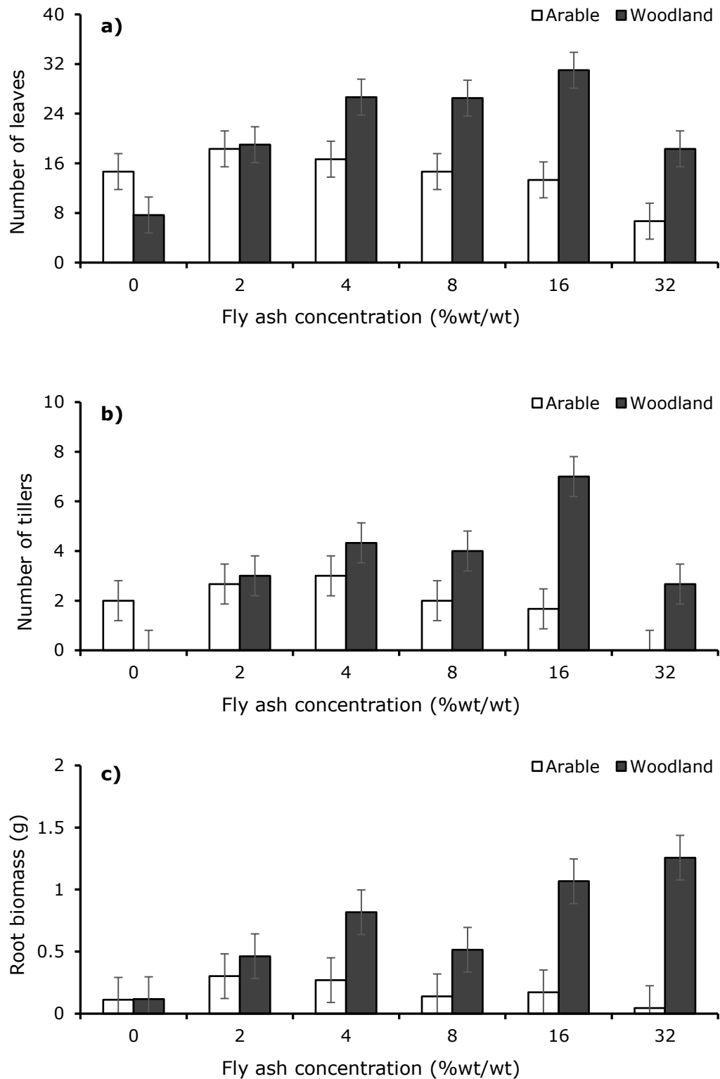
Figure 6-2: Effect of UK ash application on a) number of leaves, b) number of tillers and c) root biomass of wheat grown in woodland and arable soils. Individual error bars are based on the pooled variance estimate from the ANOVA with 23 degrees of freedom. LSD for number of leaves =8.47, number of tillers =2.35 and root biomass =0.53
