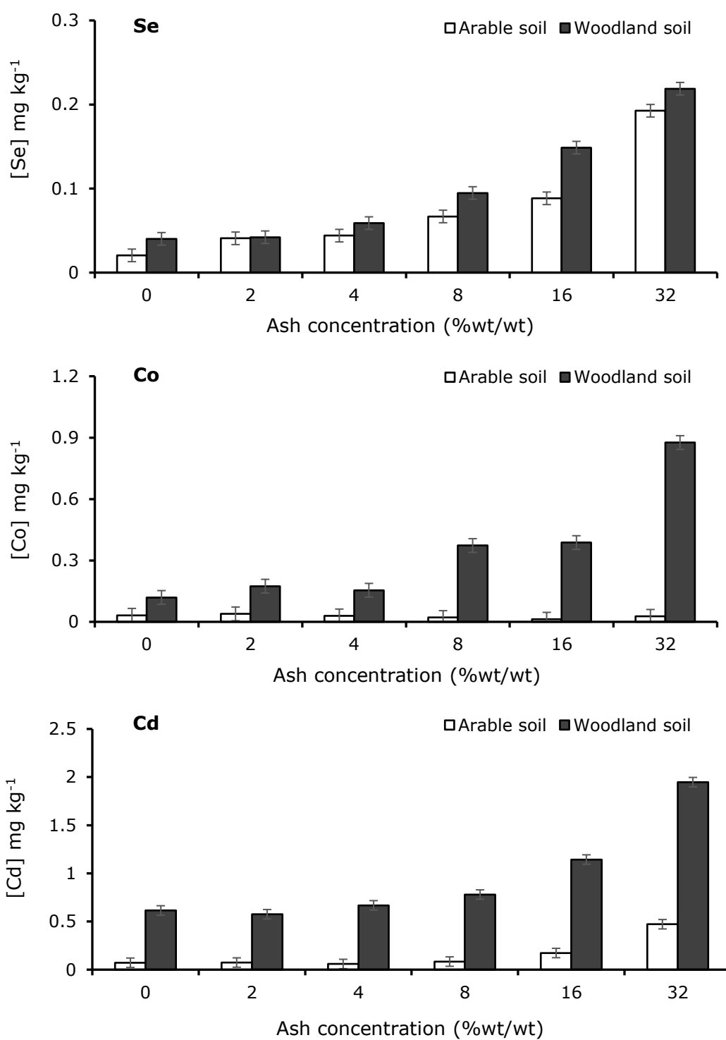
Figure 6-20: Total concentration of PTEs in wheat shoots grown in woodland and arable soil amended with ash. Individual error bars are based on the pooled variance estimate from the ANOVA with 33 degrees of freedom. LSD (for interaction term) for Se=0.022, Co=0.097 and Cd=0.14.
