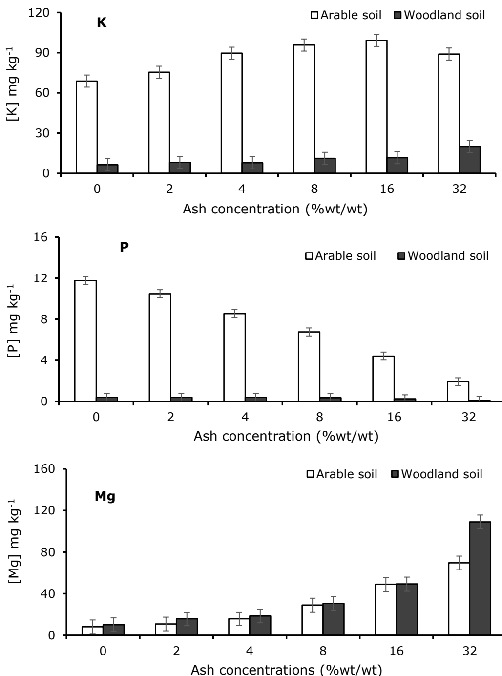
Figure 6-14: The effect of coal ash on water extractable nutrients in woodland and arable soils. Individual error bars are based on the pooled variance estimate from the ANOVA with 33 degrees of freedom. LSD (for interaction terms) for K= 12.99, P= 1.12 and Mg= 18.88. Please take note of scale differences on Y axes.
