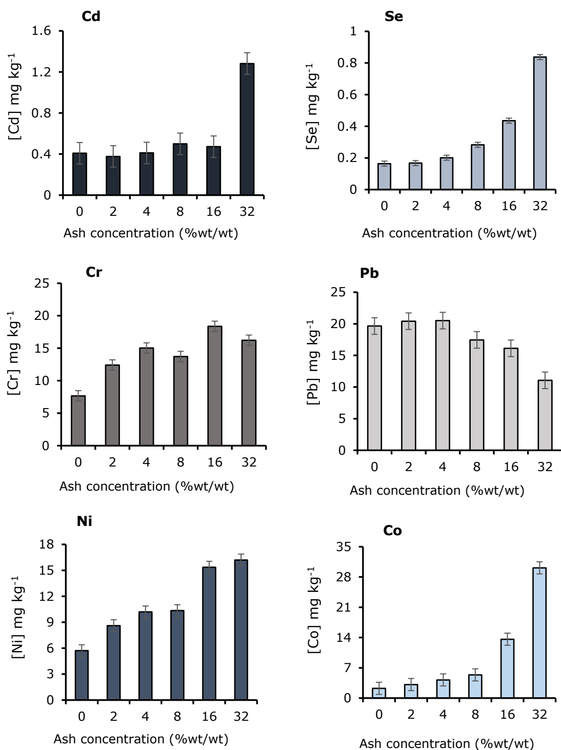
Figure 6-19: Total concentration of PTEs in wheat roots grown in soil amended with ash. Data are means pooled across woodland and arable soils. Individual error bars are based on the pooled variance estimate from the ANOVA with 33 degrees of freedom. LSD (for ash as a single factor) for Cd=0.301, Se=0.046, Cr=2.30, Pb=3.77, Co=4.03 and Ni=1.98.
