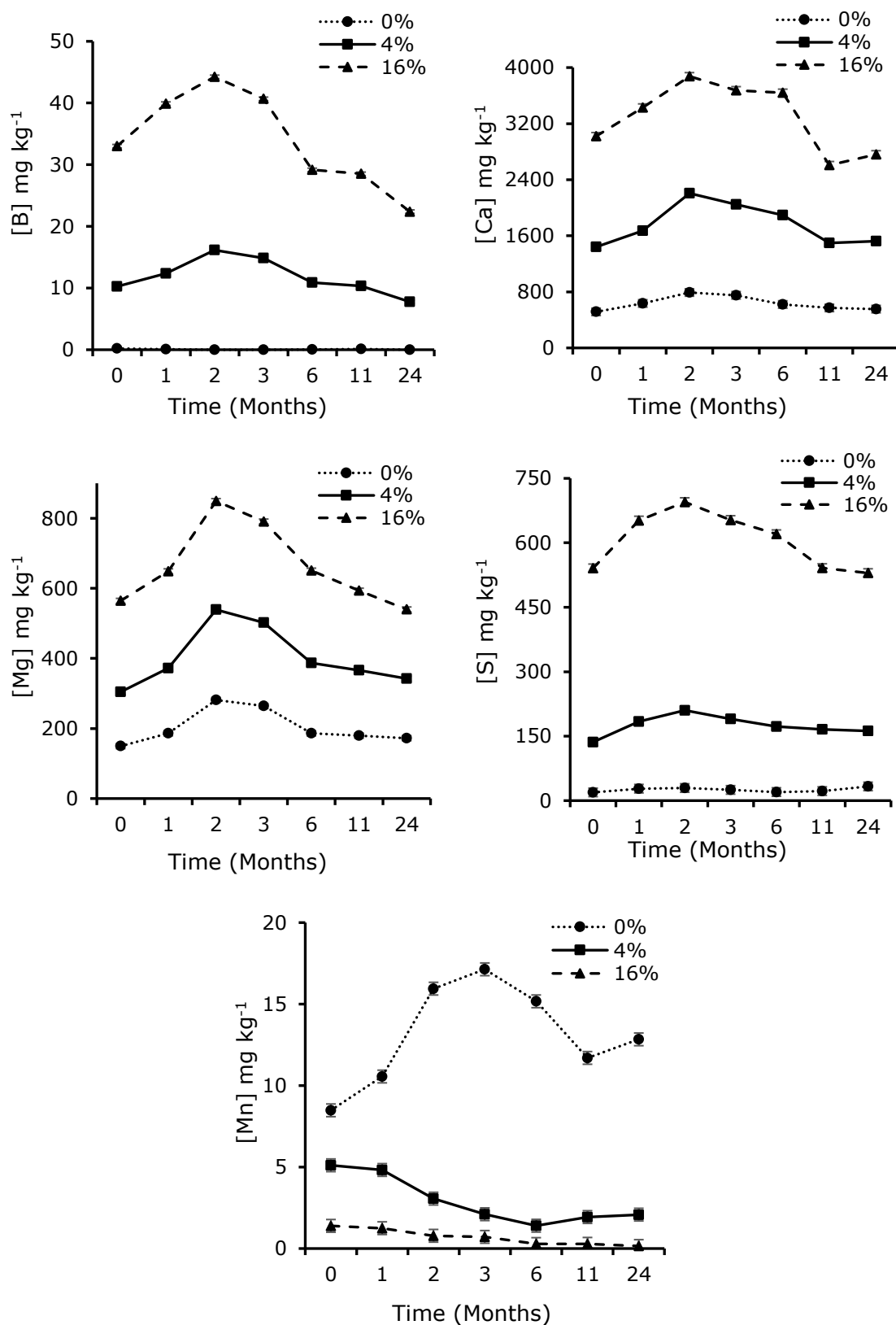
Figure 4-7: Ash induced changes in exchangeable nutrient concentrations (B, Ca, Mg, S and Mn) following soil incubation for 24 months. Individual error bars are based on the pooled variance estimate from the ANOVA with 63 degrees of freedom. LSD for B=0.8063, Mg=20.16, Ca=149.1, S=27.97 and Mn=1.1005
