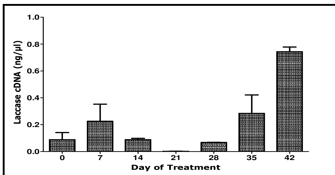
Figure 35: A qPCR quantification of laccase gene transcripts using laccase specific primers Lac2Fa/Lac2Ra on GBLS-inoculated T3 oil palms using qPCR (Illumina, USA). The unit (ng/ \mu\text{l} ) was calculated by using a standard
