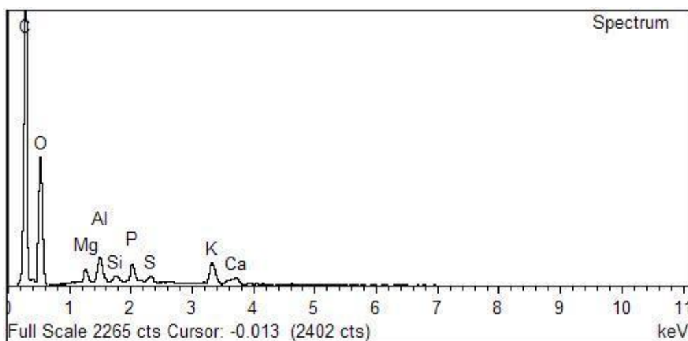
Figure 4 - 2 EDX spectrum for Jatropha curcas pressed cake
