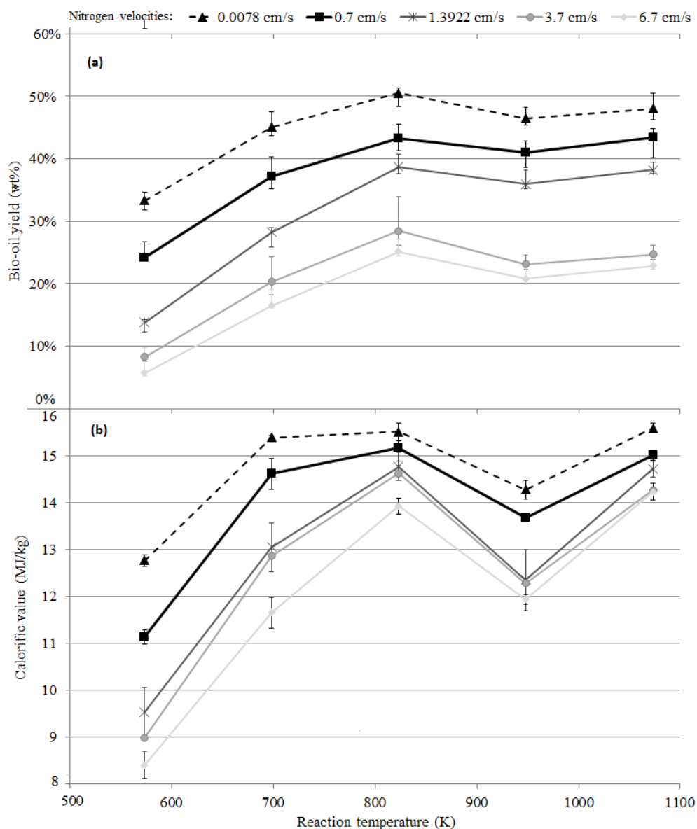
Figure 5 - 1 Effect of temperature and N 2 velocity on bio-oil (a) yield, (b) and calorific value from conventional pyrolysis
