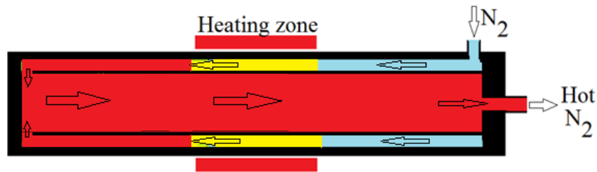
Figure 3 - 11 Annulus pre-heater
