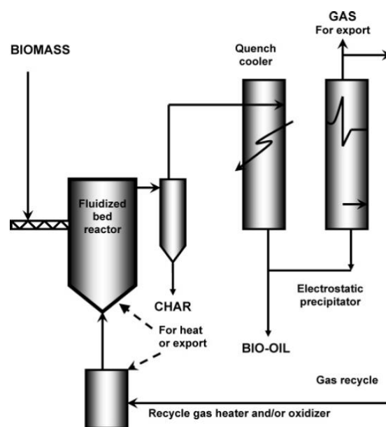
Figure 2 - 11 Fluidised bed pyrolysis reactor [17]
