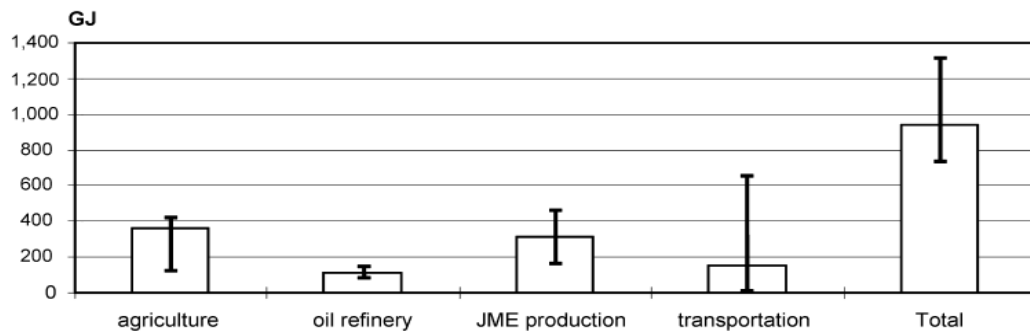
Figure 2 - 8 Energy consumption for Jatropha curcas and its products [24]
